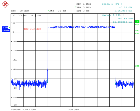
\pi/4 -DQPSK_Hopping_2DH3 1.662ms
