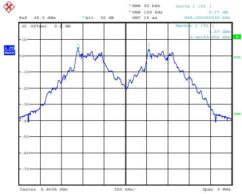
GFSK_Low 0.996MHz
