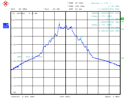
GFSK_Middle 0.831MHz
