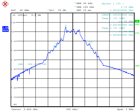
GFSK_Low 0.831MHz
