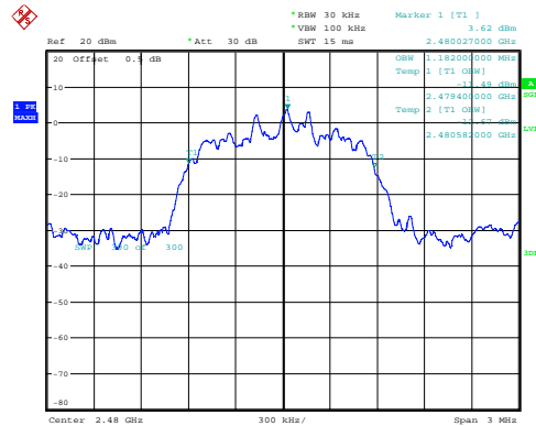
\pi/4 -DQPSK_High 1.182MHz
