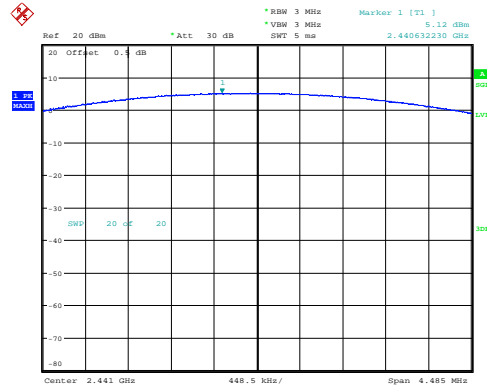
GFSK_Middle 5.12dBm
