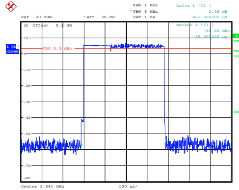
\pi/4 -DQPSK_Hopping_2DH1 0.402ms
