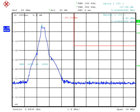
GFSK_High 57.69dB
