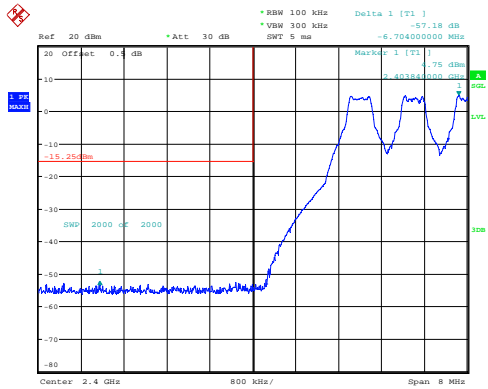
GFSK_Hopping_Lower 57.18dB
