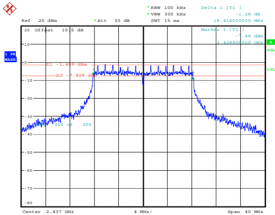
g_2437MHz 16.416MHz
