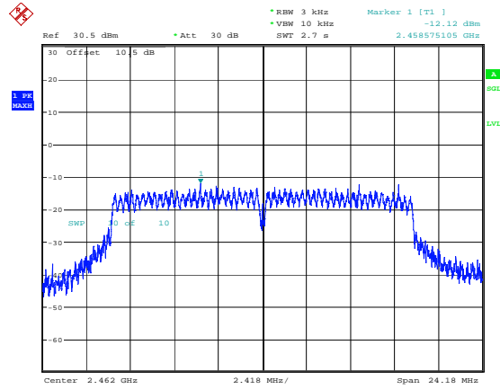
g_2462MHz -12.12dBm/3kHz
