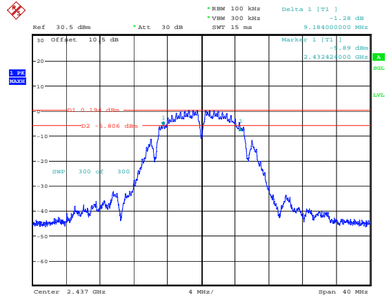
b_2437MHz 9.184MHz
