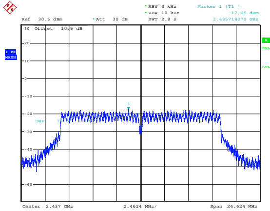
g_2437MHz -17.65dBm/3kHz
