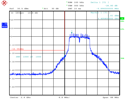
g_2412MHz 26.80dB
