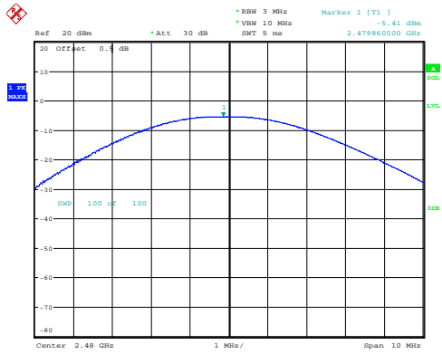
High -5.41dBm
