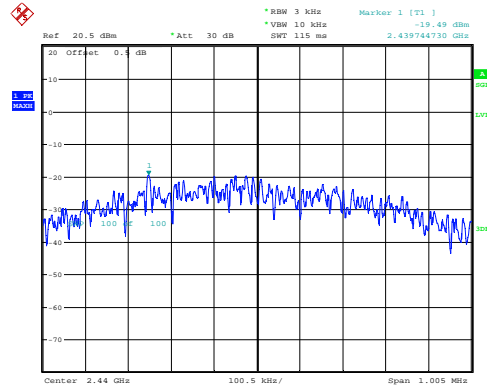
Middle -19.49dBm/3kHz
