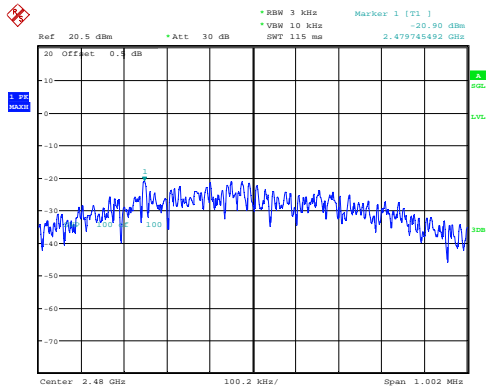
High -20.90dBm/3kHz
