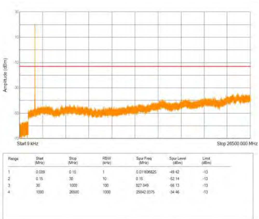
Band66 QPSK BW=10MHz Channel=132322 RB Size=50 Position=#0
