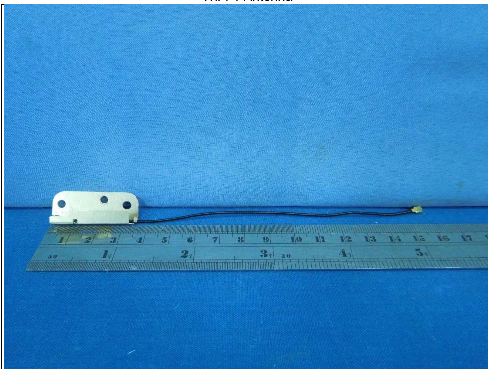
WiFi-1 Antenna
