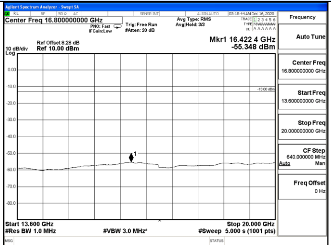
13.6 GHz – 20 GHz
