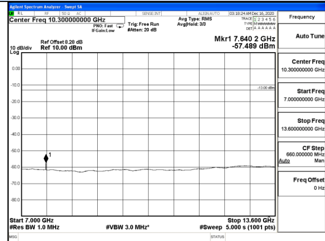
7 GHz – 13.6 GHz
