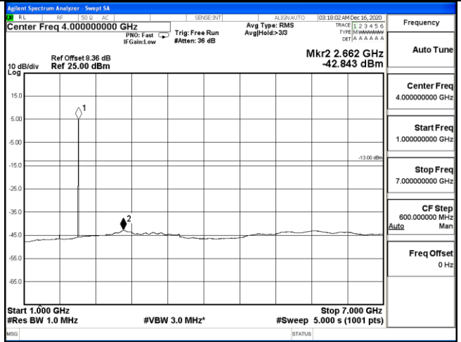
1 GHz – 7 GHz
