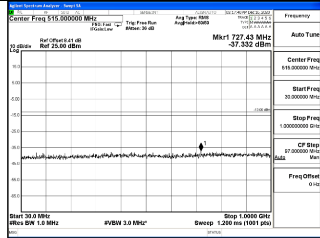
30 MHz – 1000 MHz
