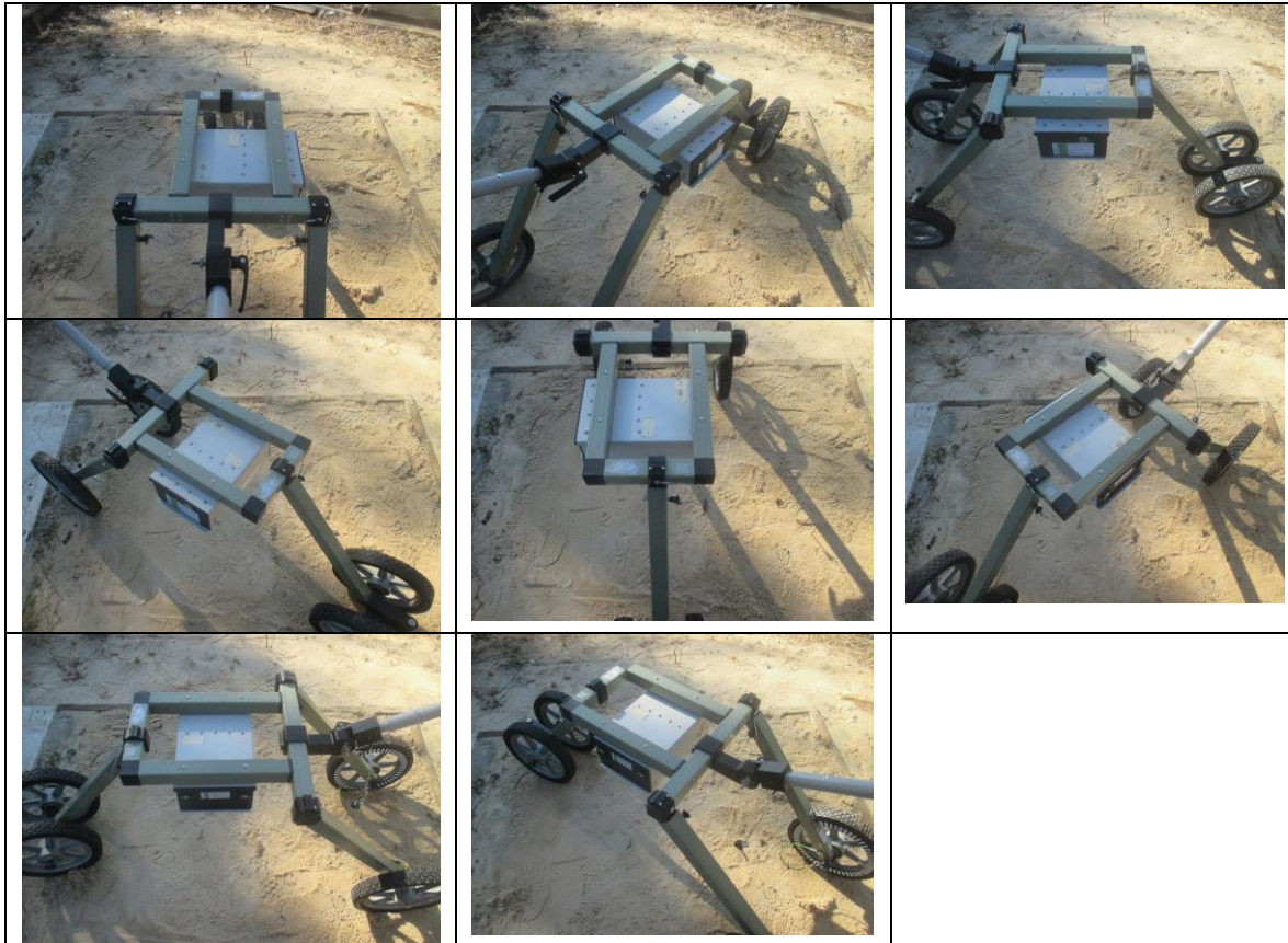
EUT Positions with 45 Degree Interval
