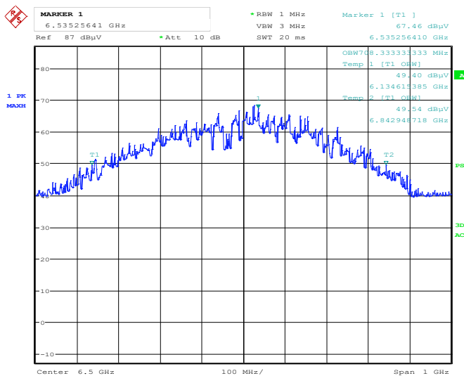
Figure 8.2-1: -10 dB bandwidth
