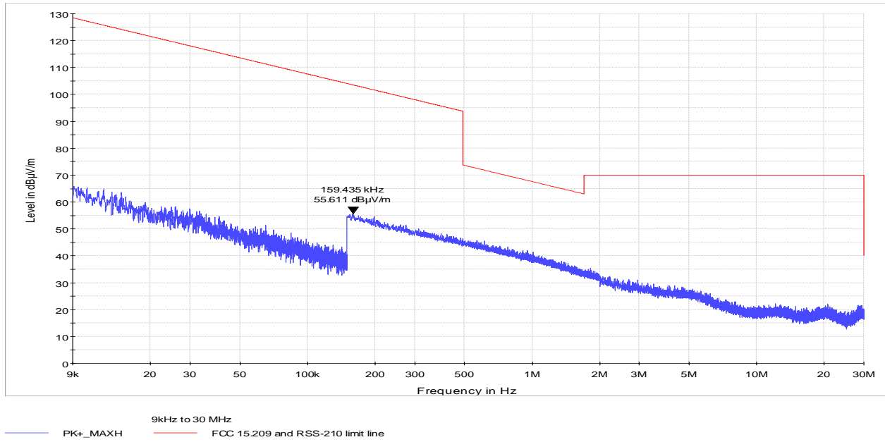
Figure 8.3-1: Radiated spurious emissions within 9 kHz to 30 MHz
