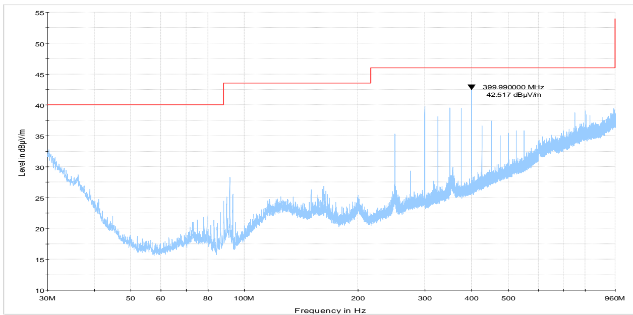
Figure 8.3-2: Radiated spurious emissions within 30–960 MHz
