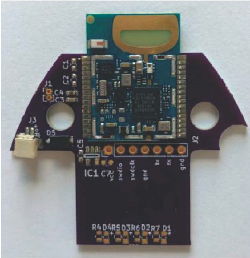
TOF RTLS ASSET TAG WITHOUT SHIELD – FRONT
