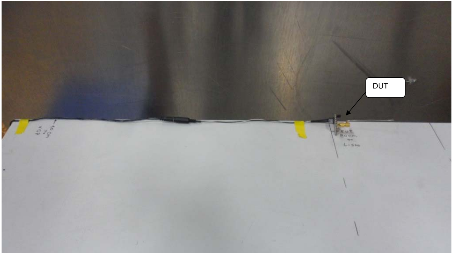
Figure E20.6 – Setup Photo – Power Line Conducted Measurements
