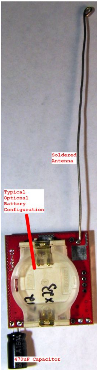
Figure E18.2 – External Photo – Module Bottom
