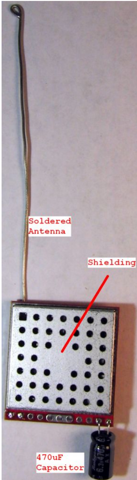
Figure E18.1 – External Photo – Module Top
