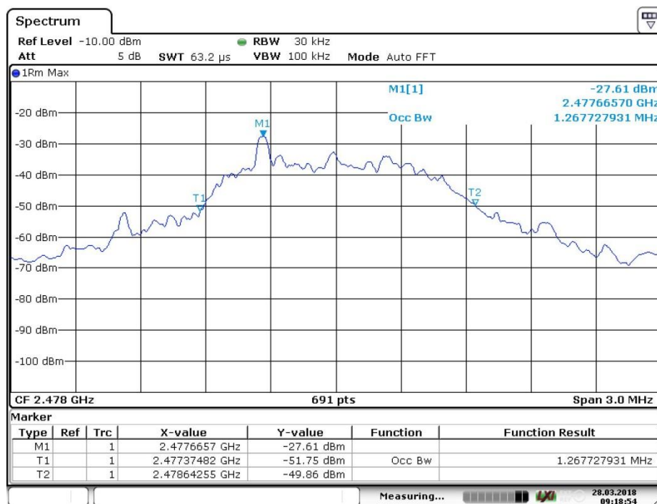
Screenshot: 99 % bandwidth Measurement, high channel
