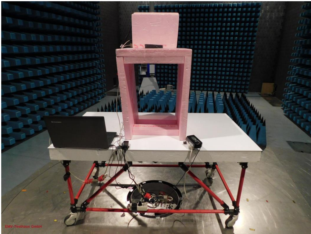
Picture 5: SAC, radiated emission test >1 GHz (front view)
