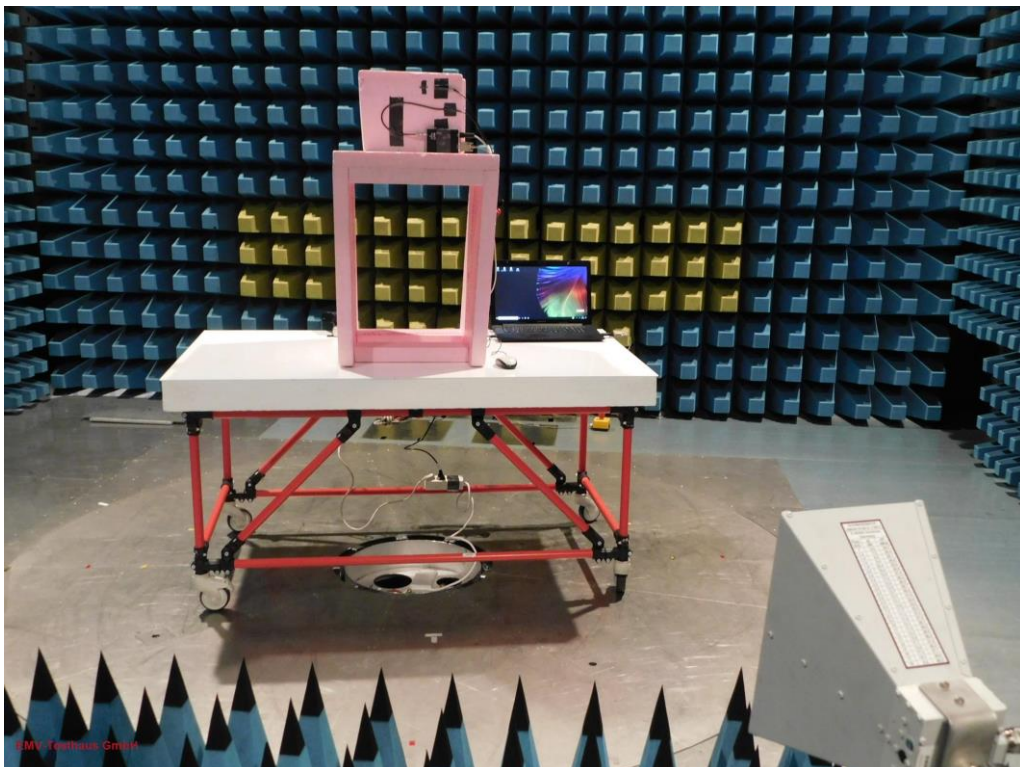
Picture 6: SAC, radiated emission test >1 GHz (rear view)
