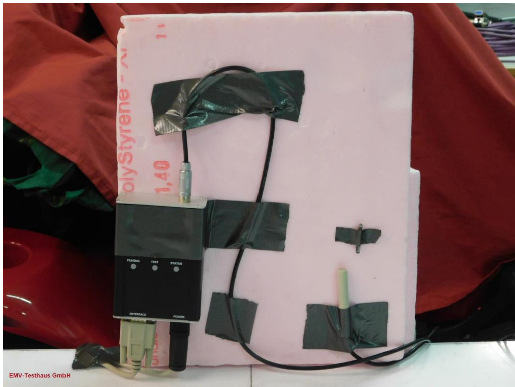
Picture 11: EUT-position 3
