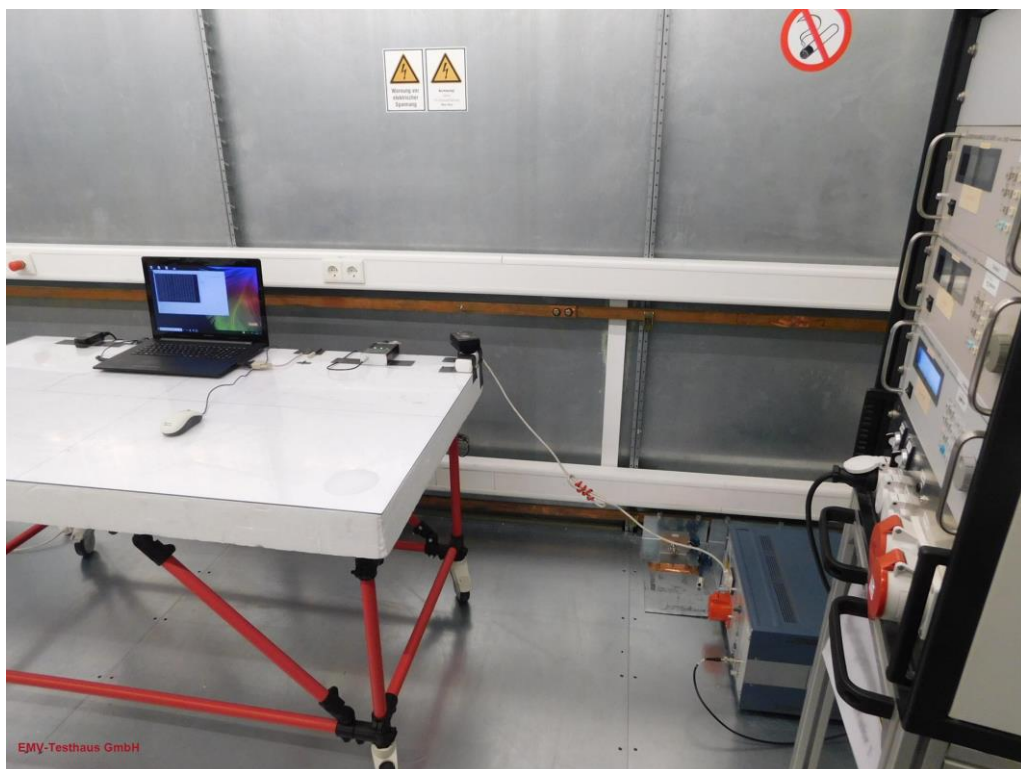
Picture 7: Test setup AC power line conducted emissions (front view)
