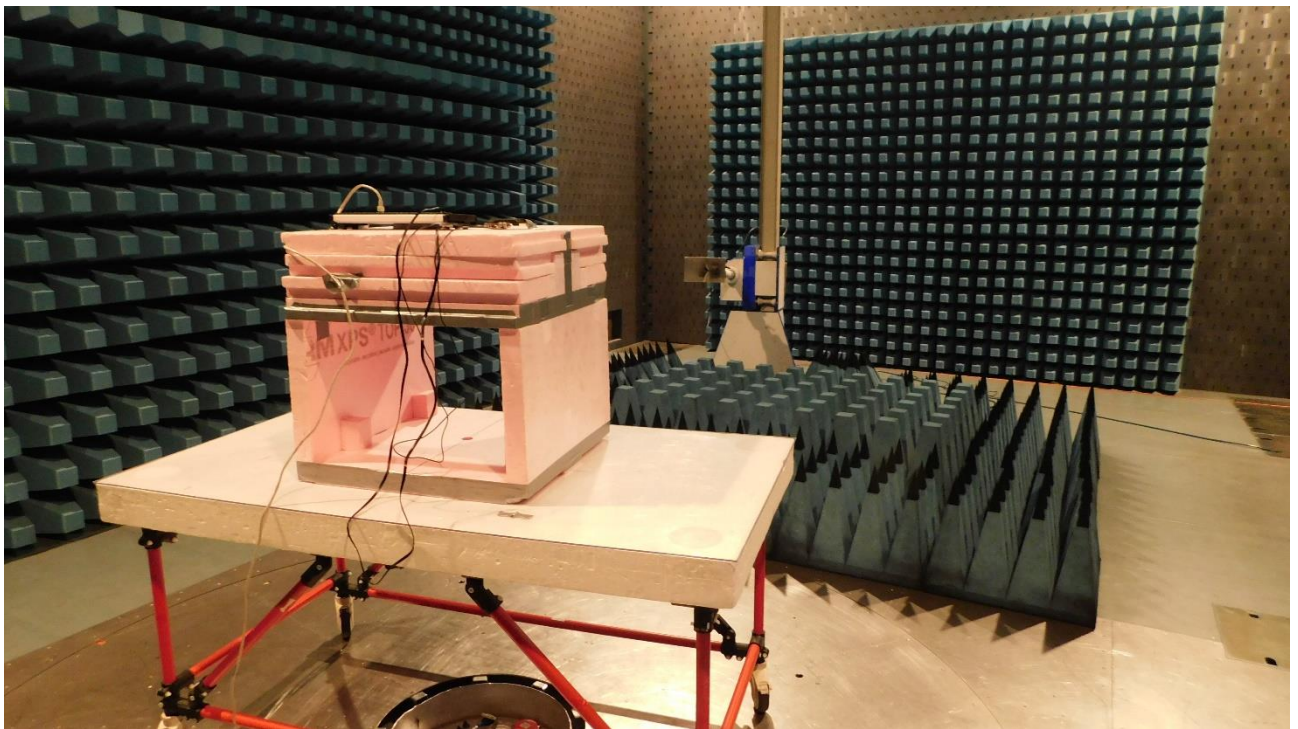
Picture 5: SAC, radiated emission test 1 GHz – 2 GHz (front view)
