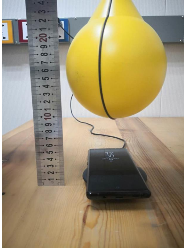
Measurement form the top of the primary/client pair
