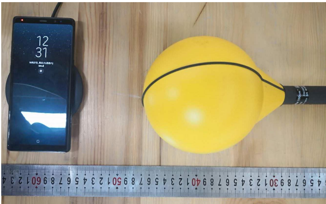
Measurement form the side of the primary/client pair
