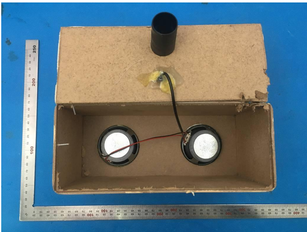
SUB-SPEAKER OPEN VIEW OF EUT
