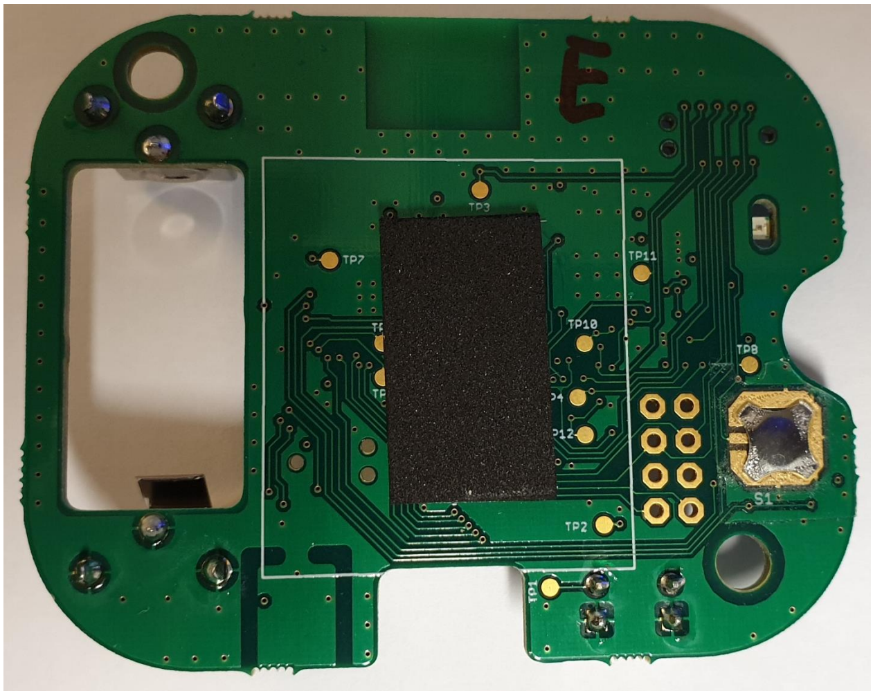
FS-TDX-03 PCB rear side view
