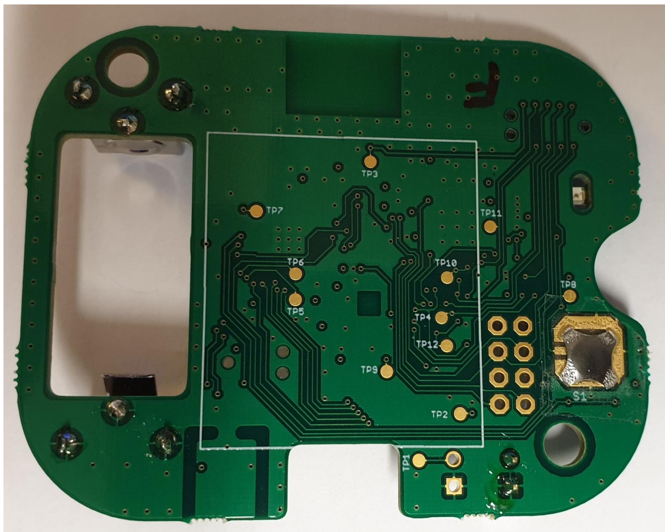
FS-TSX-03 PCB rear side view
