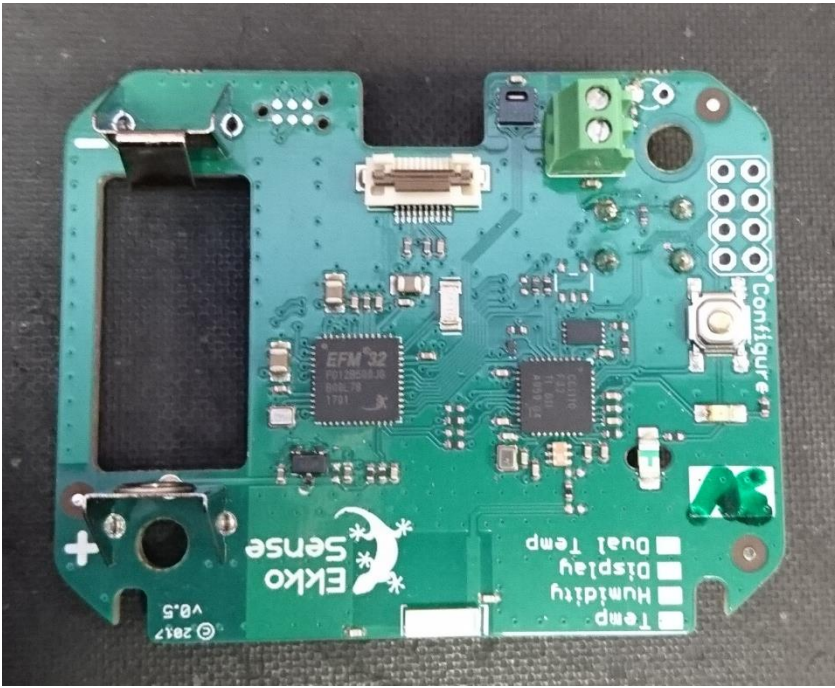
PCB component side view
