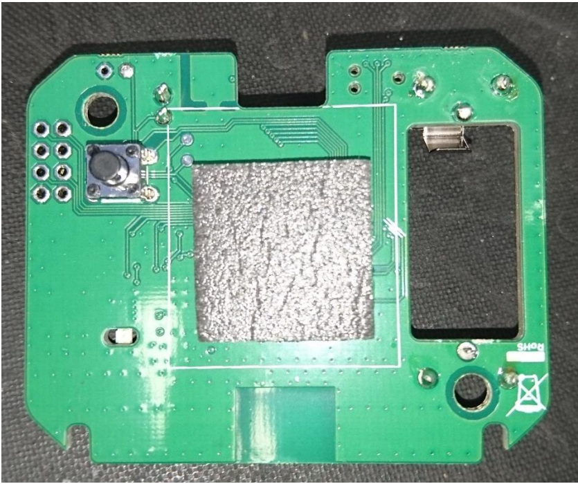
PCB component side view
