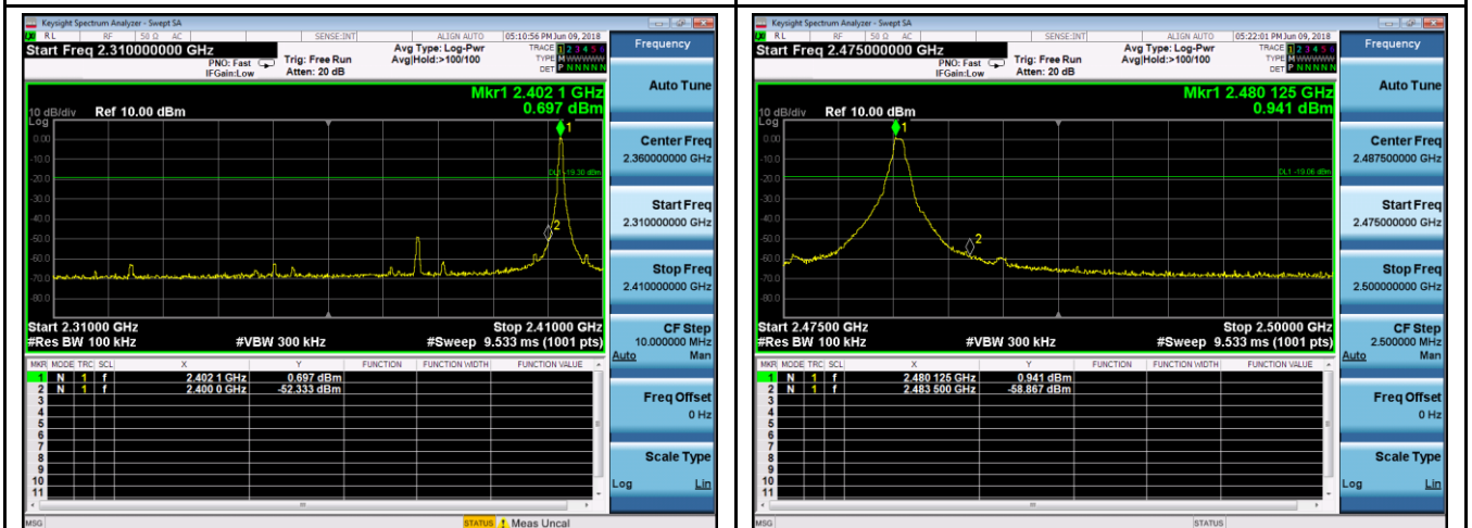
GFSK-Left Side
