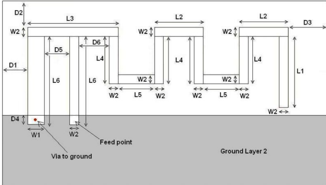
Figure 3: Antenna Dimensions
