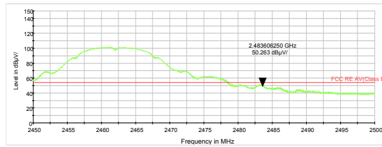
802.11b-Channel 11 Average
