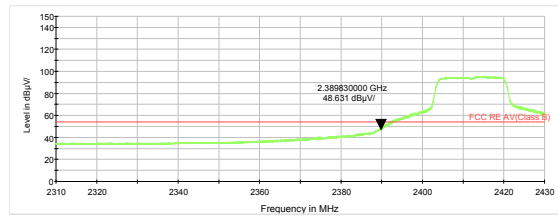
802.11g-Channel 1 Average
