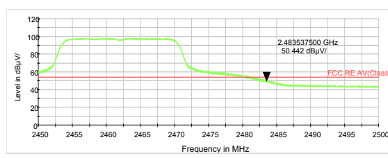
802.11g-Channel 11 Average
