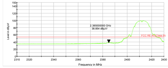
802.11b-Channel 1 Average
