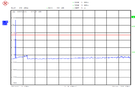
NB-IOT Band 4 CH-Low 1GHz ~20GHz
