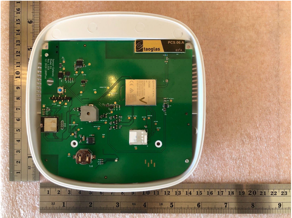
G1 Interior photo with module shields
