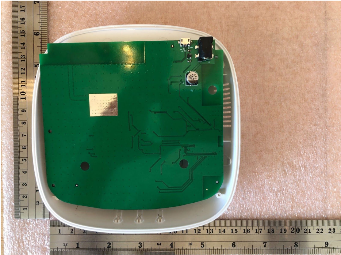
G1 PCBA bottom showing power and USB interfaces
