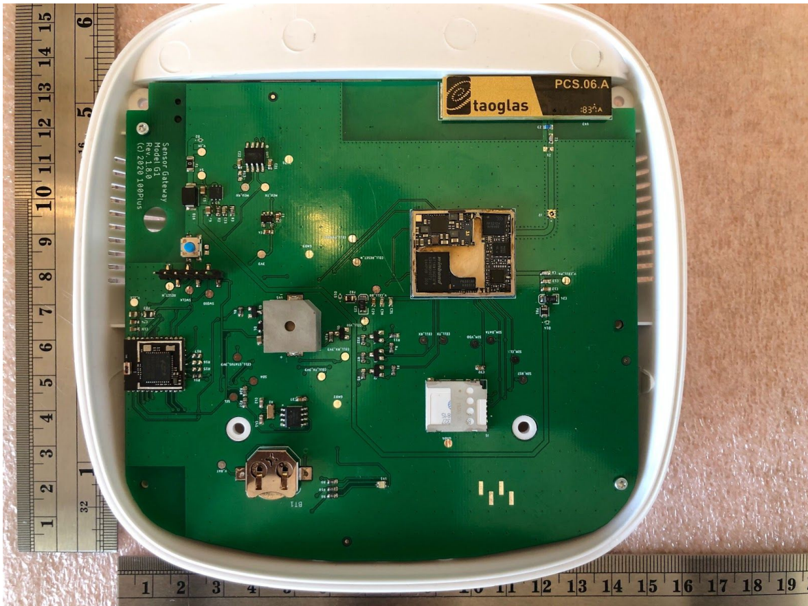
G1 Interior photo without module shields
