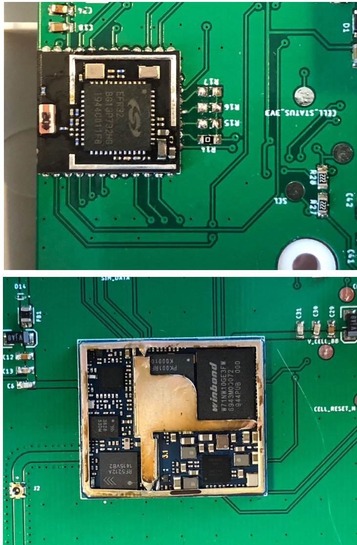
G1 detail of BLE module (top) and LTE module (bottom)
