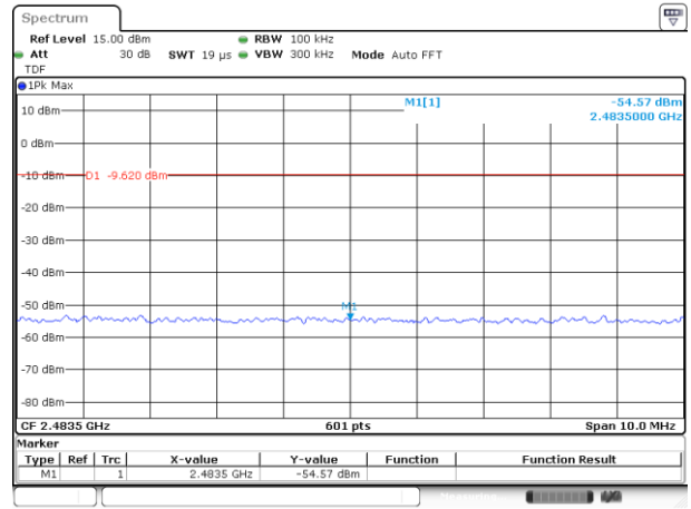
802.11b Middle Channel (right), Band Edge
