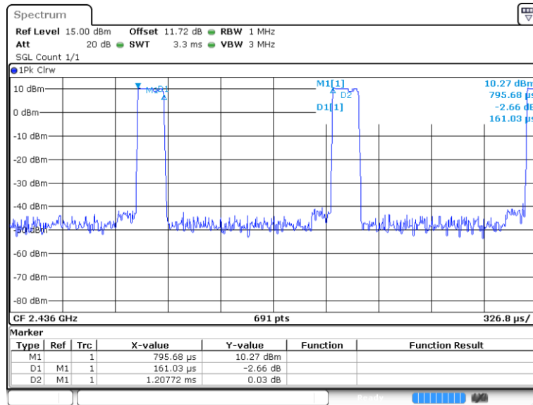
GFSK on time/100 ms (One Pulse) Plot on Middle Channel
