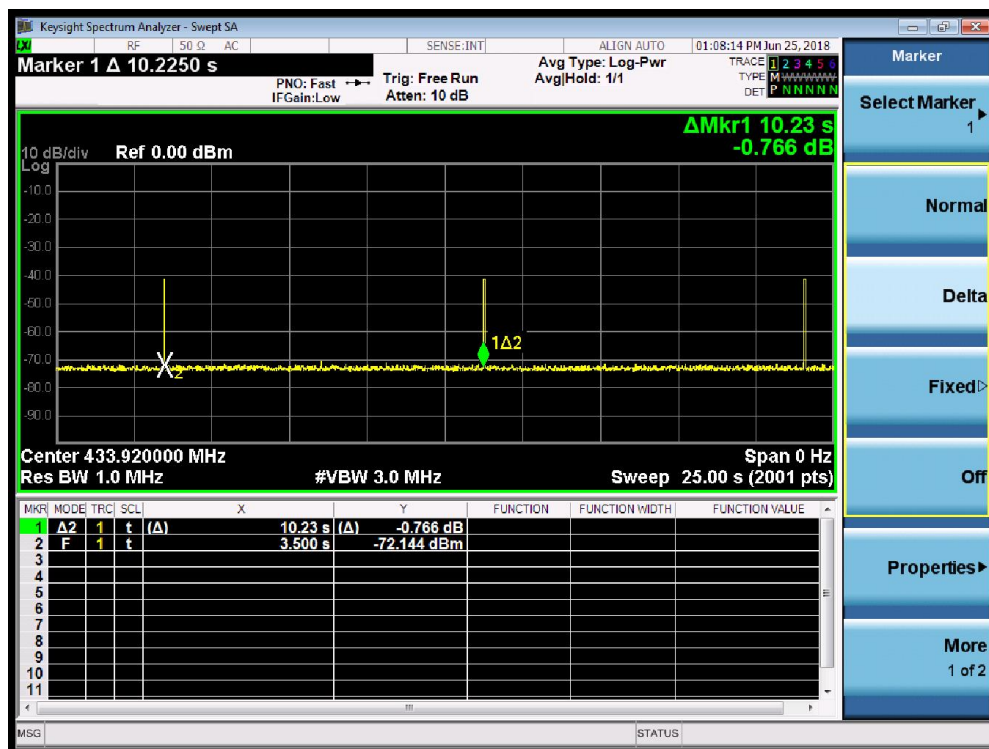
Silent Time for 433.92MHz FSK
