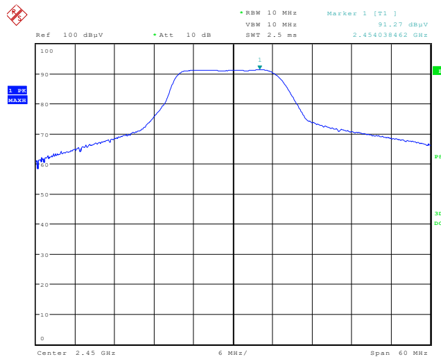
PK detector is for PK value
