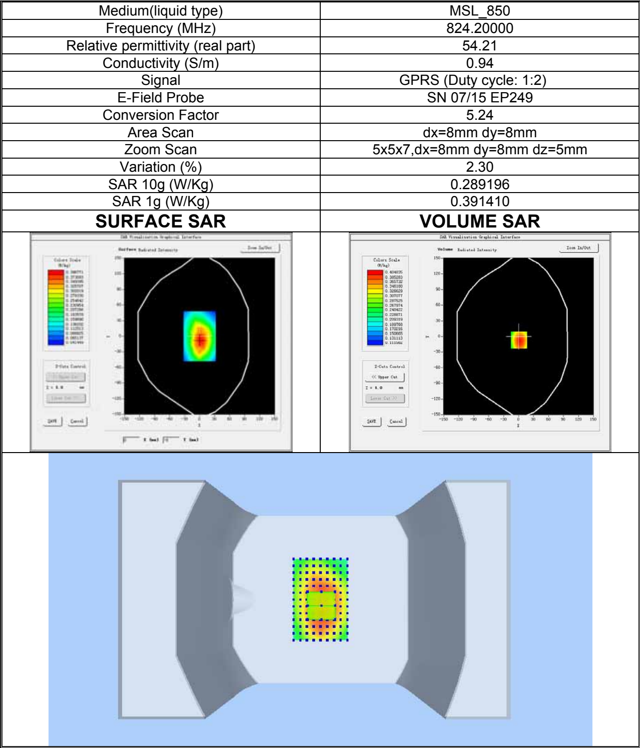
Plot 7: GPRS850MHz, Low channel(Body-worn, Right edge) Product Description: Mobile Phone Test Date: 2018-06-23
