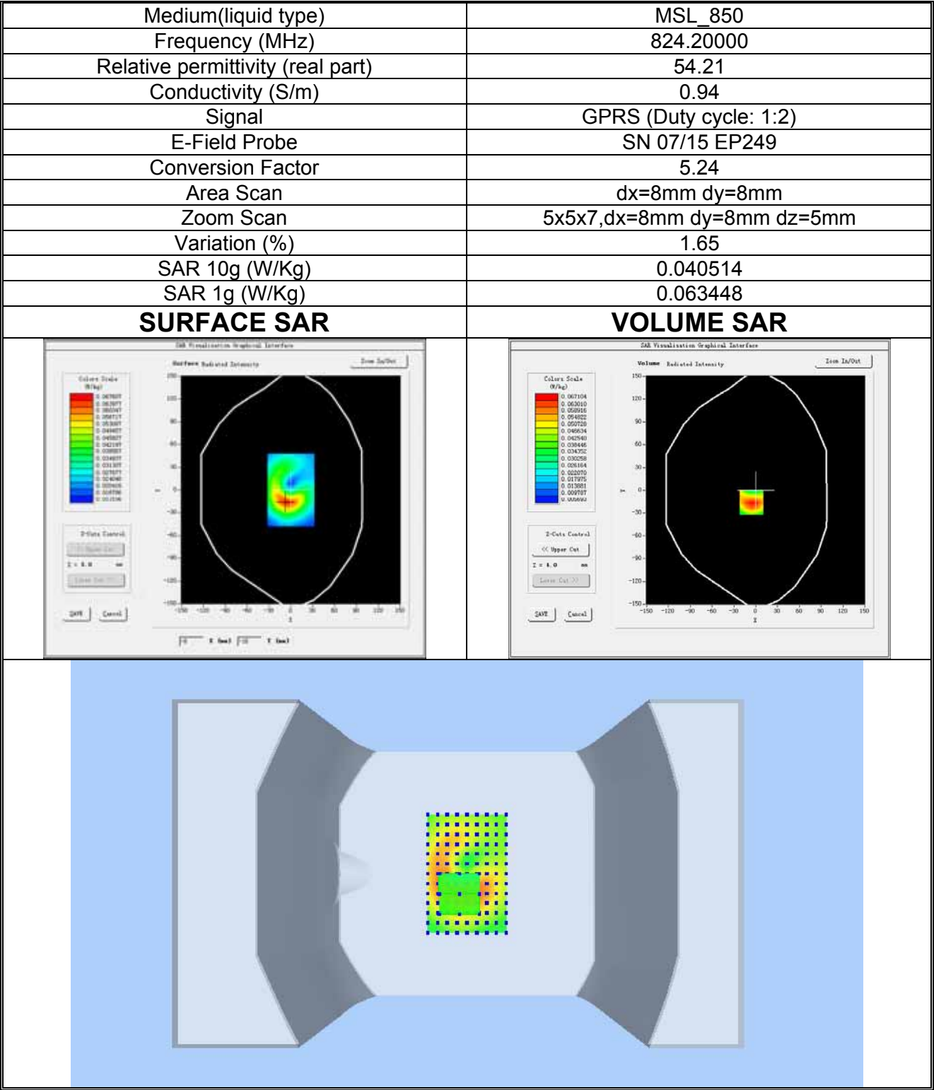
Plot 8: GPRS850MHz, Low channel(Body-worn, Bottom edge) Product Description: Mobile Phone Test Date: 2018-06-23
