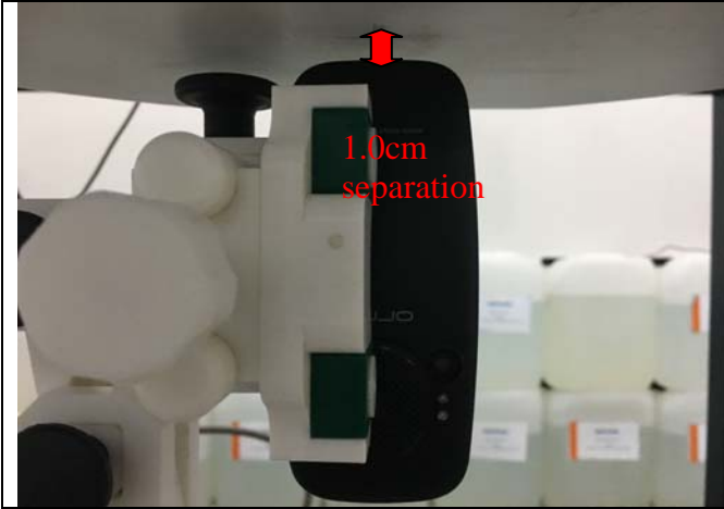
Body-Worn(Bottom edge)
