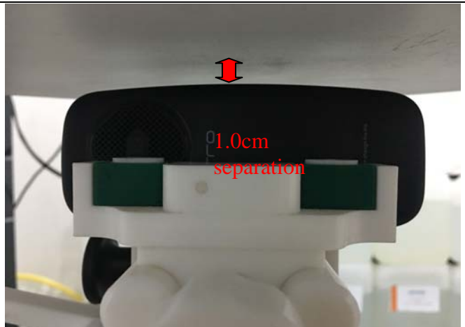
Body-Worn(Left edge)
