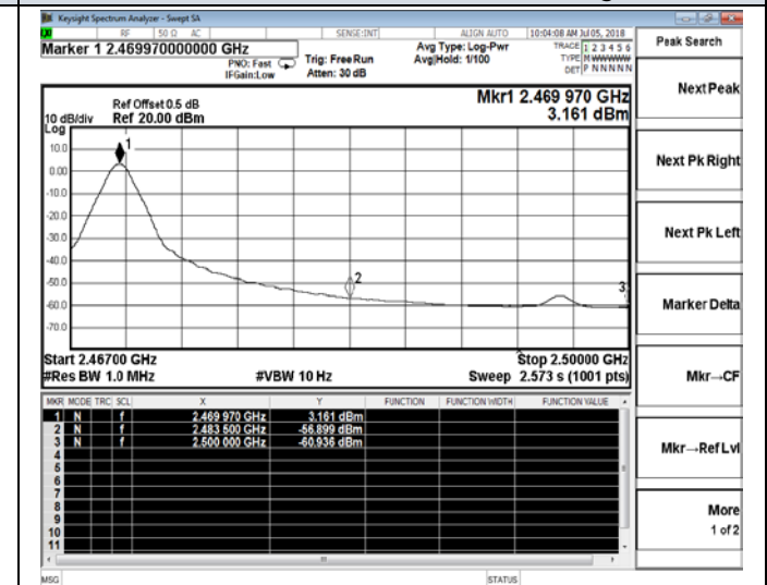
High Channel / 2470MHz – Average
