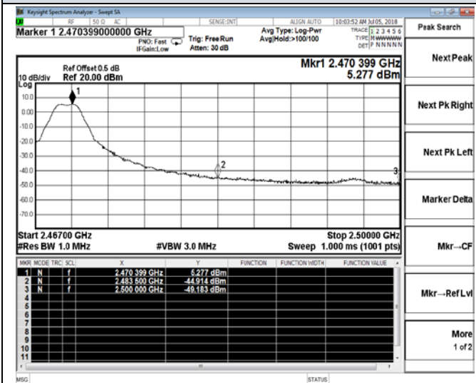
High Channel / 2470MHz - Peak
