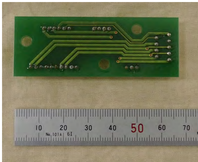
(h) Carriage junction board A – Bottom side
