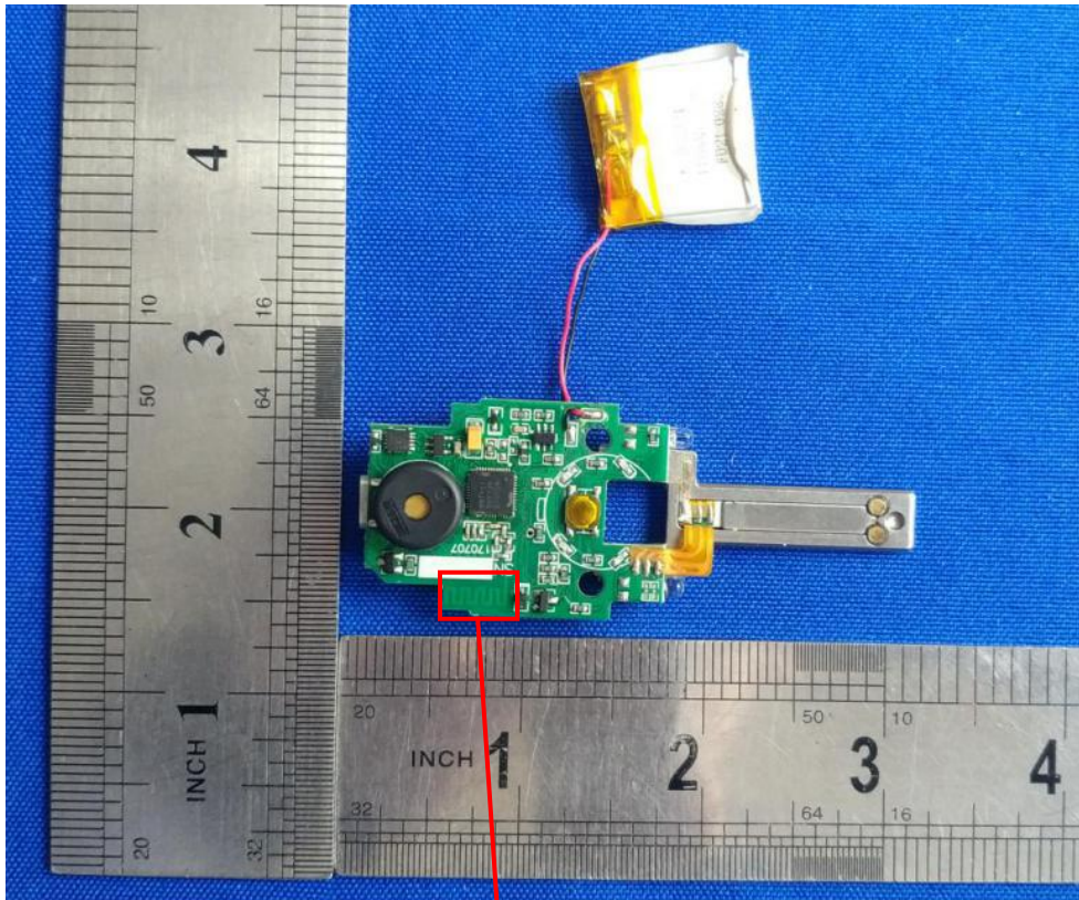
PCB antenna
