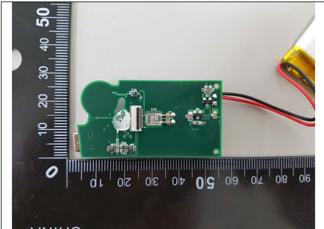
Power Board Rear
