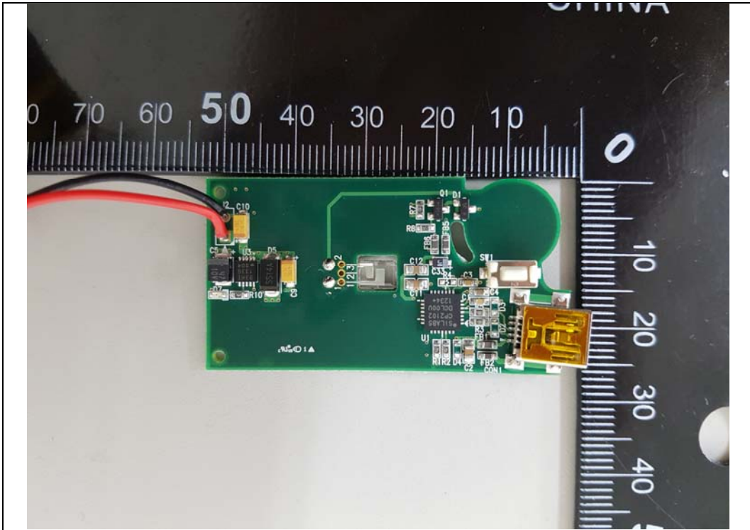
Power Board Front
