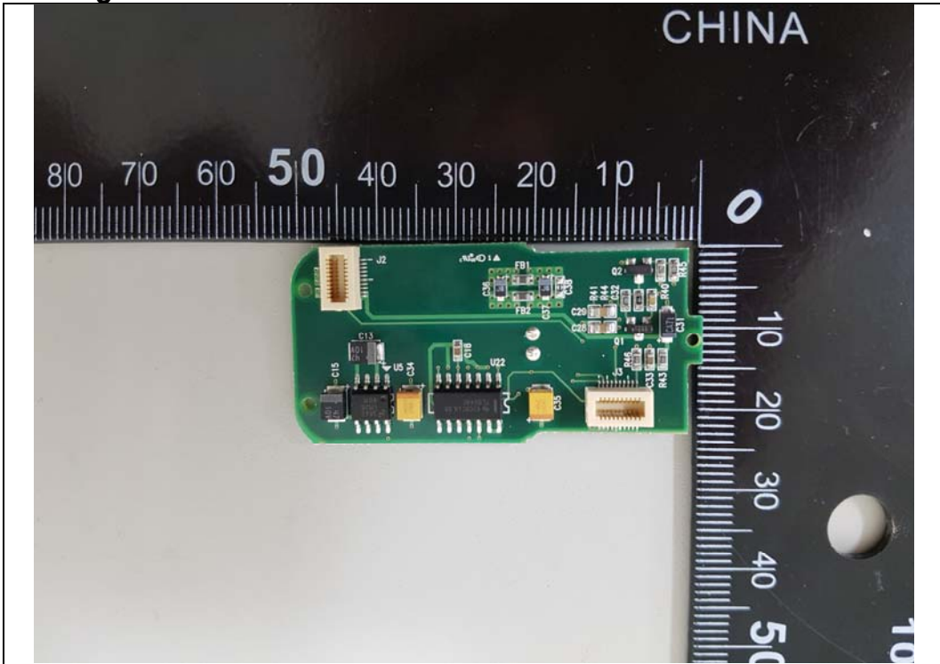
Analog Board Front
