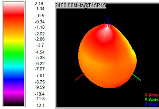
© 3D Gain Pattern (2400 MHz)
