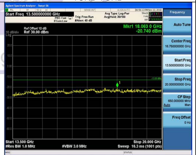
13.5GHz~20GHz
