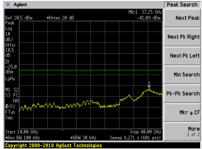
Low Channel 5860 MHz Chain 0, 10GHz – 40GHz
