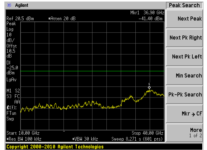
Middle Channel 5890 MHz Chain 1, 10GHz – 40GHz
