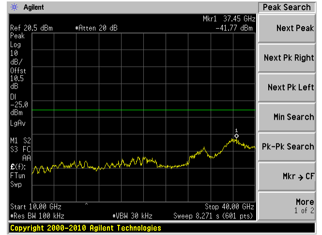
Middle Channel 5890 MHz Chain 0, 10GHz – 40GHz
