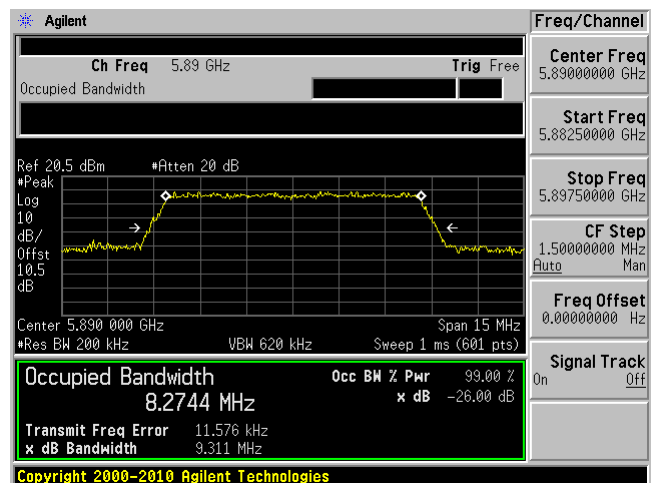
Middle Channel, 5890MHz Chain 1
