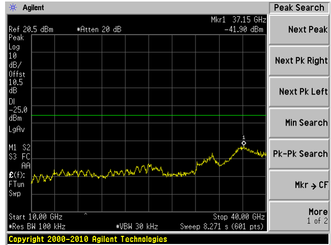
Low Channel 5860 MHz Chain 1, 10 GHz – 40GHz
