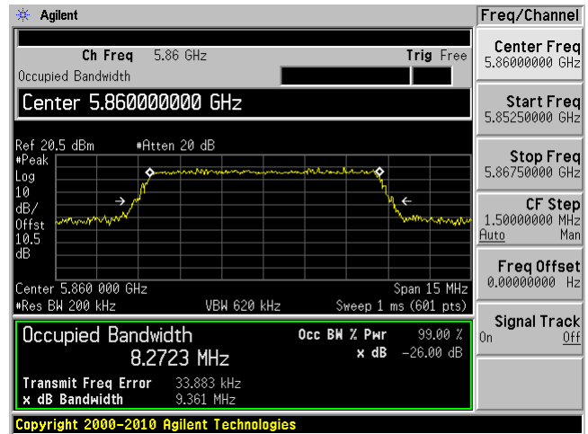
Low Channel, 5860MHz Chain 1
