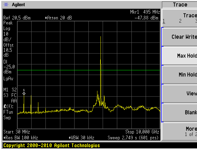
Low Channel 5860 MHz Chain 0, 30MHz – 10GHz
