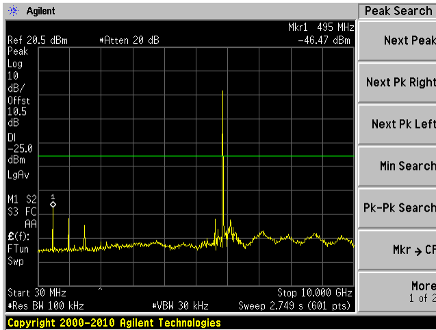
Low Channel 5860 MHz Chain 1, 30MHz – 10GHz
