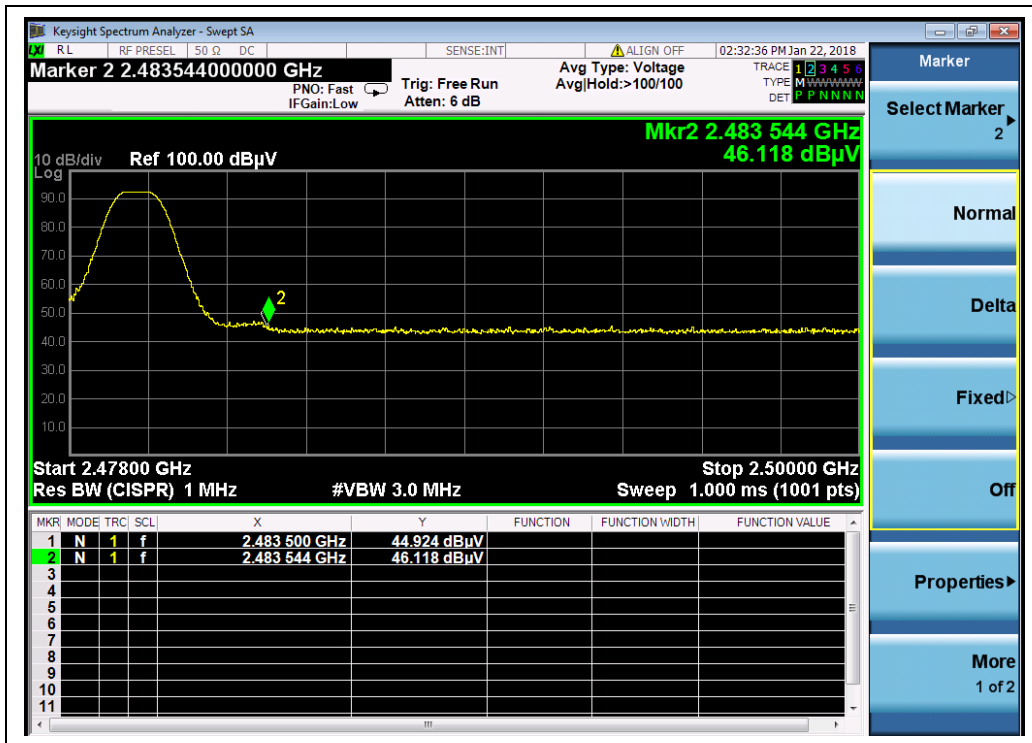
(Channel = 39, PEAK)
