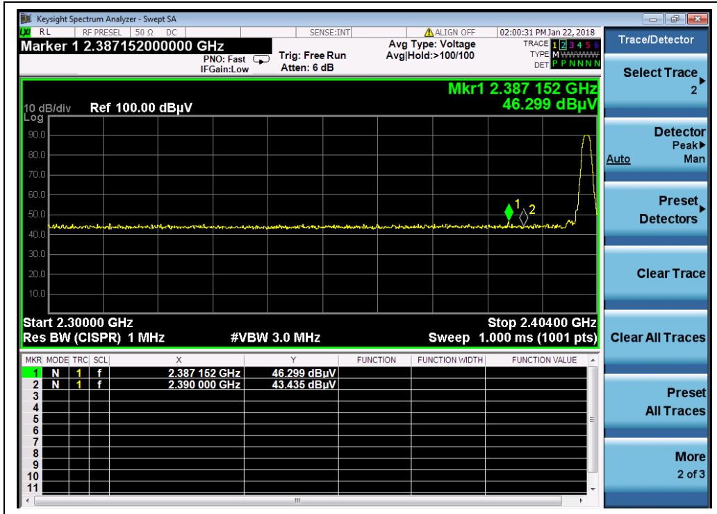
(Channel = 0, PEAK)
