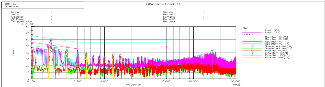
Figure 6. plot of Conducted Emission
