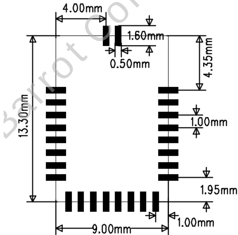
Figure 5: PCB layout Footprint
