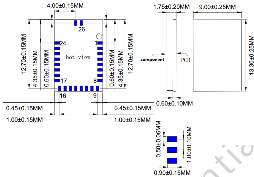
Figure 4: i410e-s Footprint
