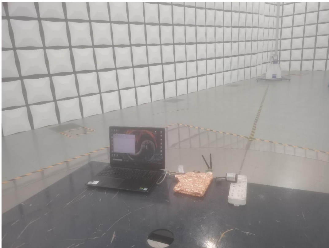
30MHz~1GHz
