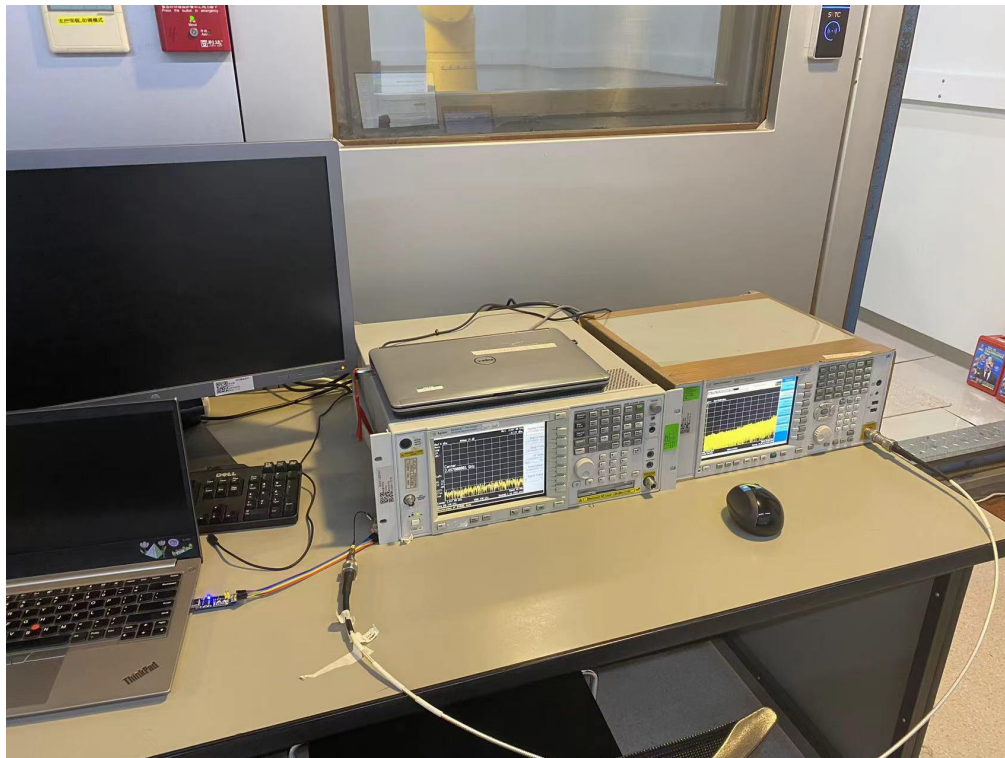
RF Conducted Test setup (BT)
