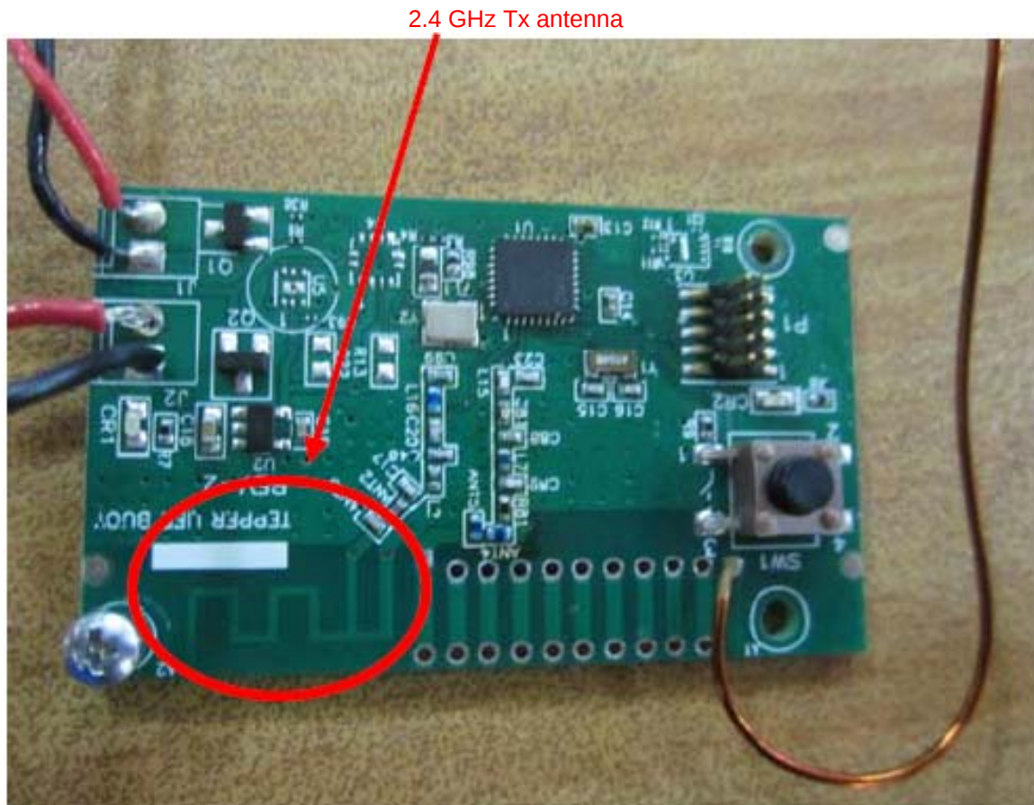
Photograph No.6 Control unit 2.4 GHz antenna
