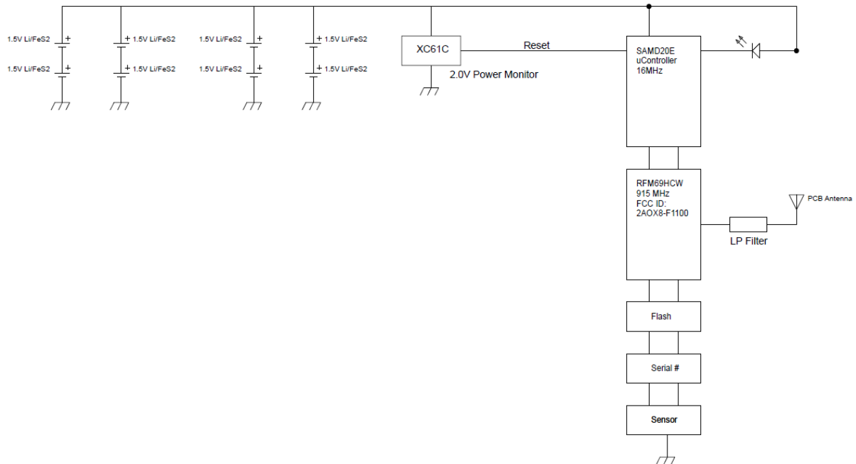
Figure 2. Flume Sensor Block Diagram.
