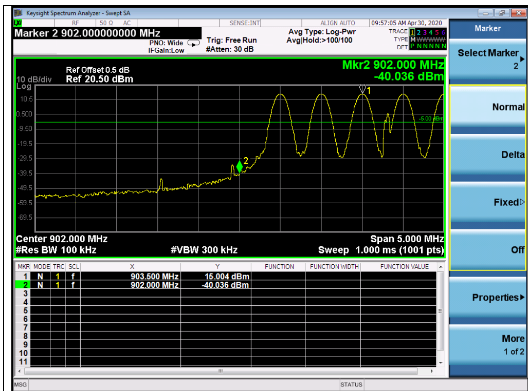
Hopping mode left side
