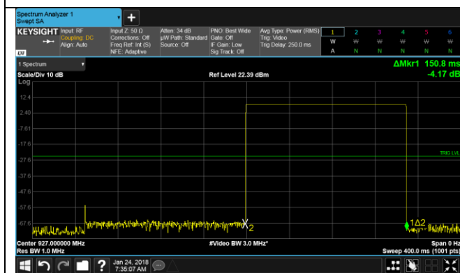
927 MHz On Time
