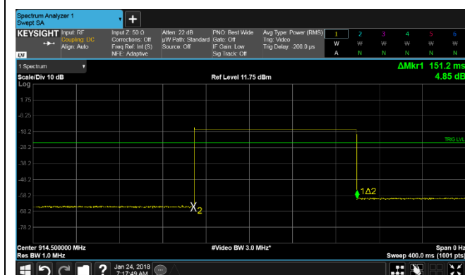
914.5 MHz On Time
