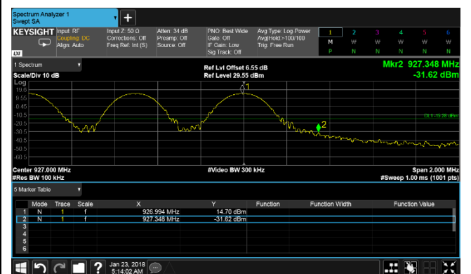
Band Edge -Hopping-927 MHz
