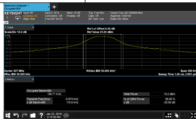
99% and 20dB BW – 927MHz
