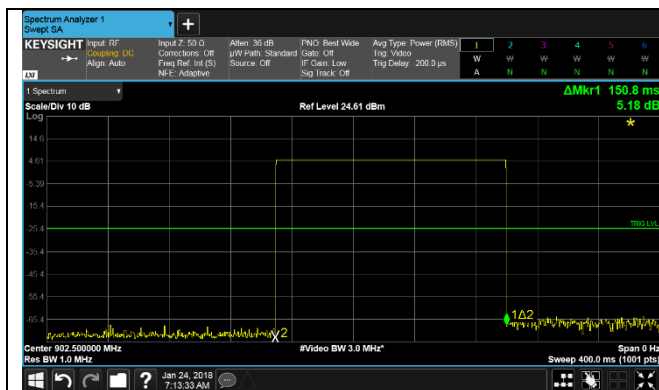
902.5 MHz On Time
