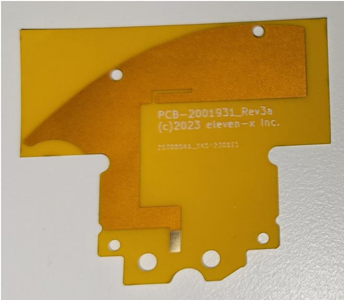
Dual Band ISM Antenna (902-928MHz & 2400-2483.5MHz) PCB top
