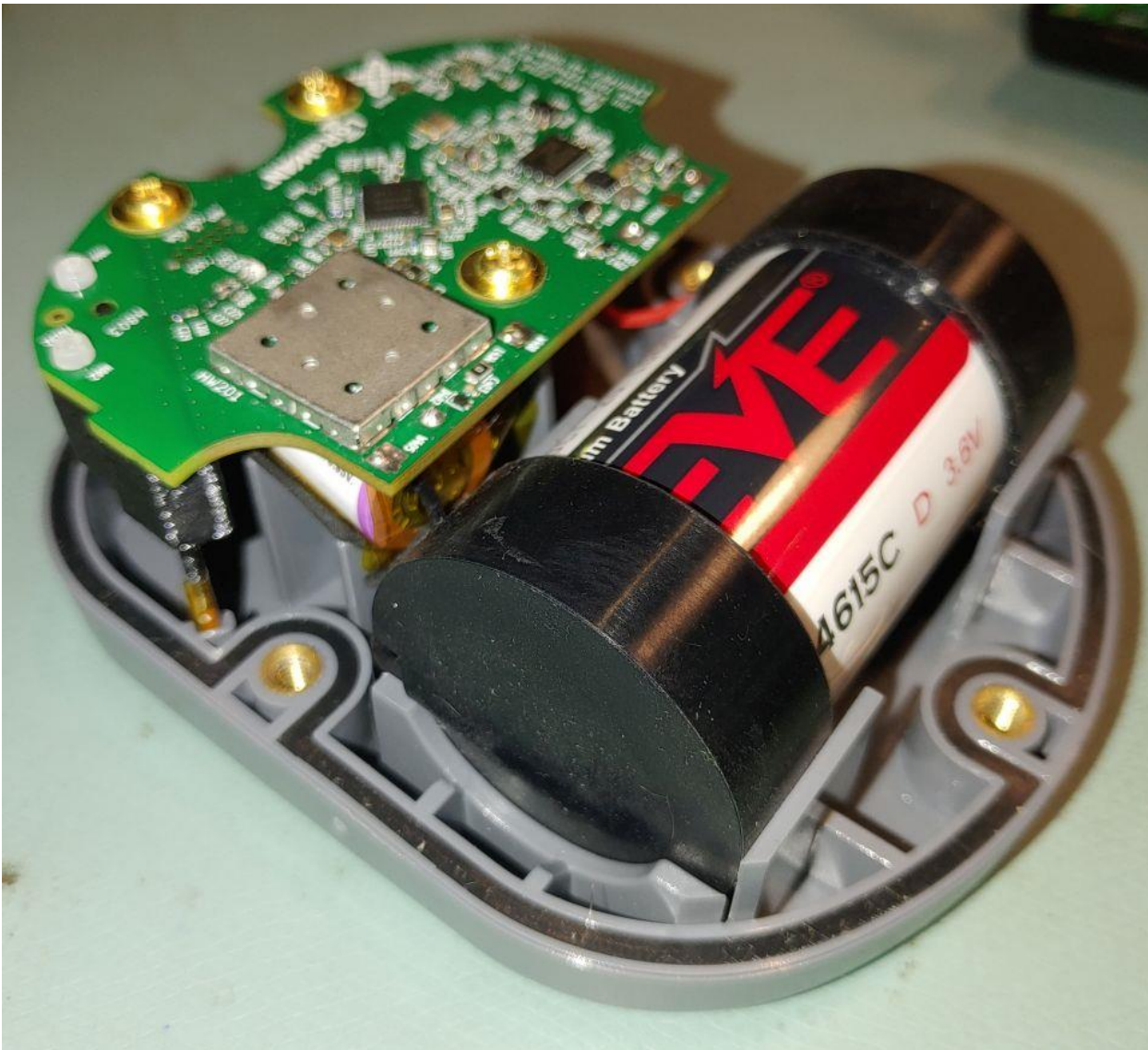
PCB with battery in enclosure top
