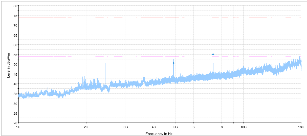
PRJ52103466 RE 1-18 GHz, BLE, mid ch., PRK002001 rev A Preview Result 1-PK+ FCC 15.209 and RSS-Gen Restricted bands peak limits FCC 15.209 and RSS-Gen Restricted bands average limits Final_Result PK+
