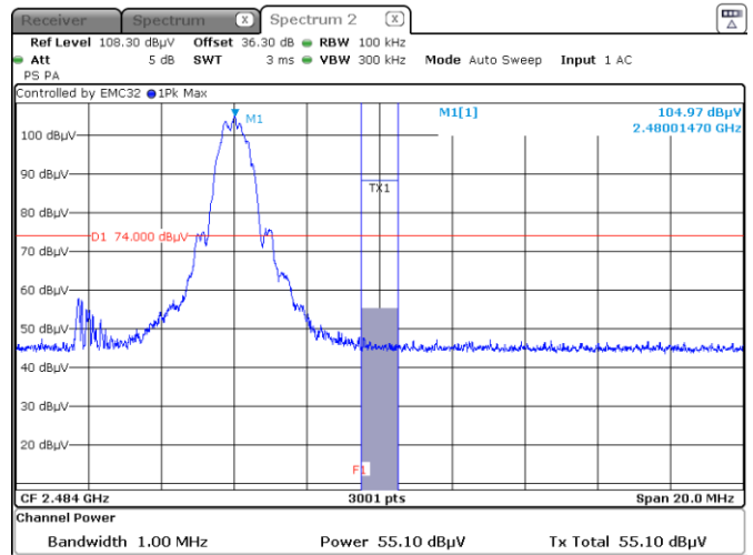
Figure 7.6-13: Radiated band edge spurious emissions at 2483.5 MHz Peak – 1 MHz
