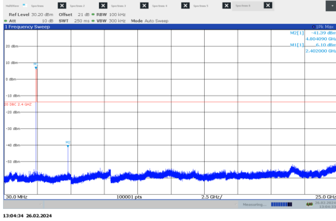
Figure 7.6-20: Conducted spurious emissions on low channel – 1 MHz
