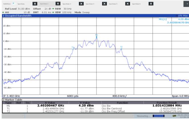
Figure 7.4-7: 99% occupied bandwidth on low channel – 1 MHz BW
