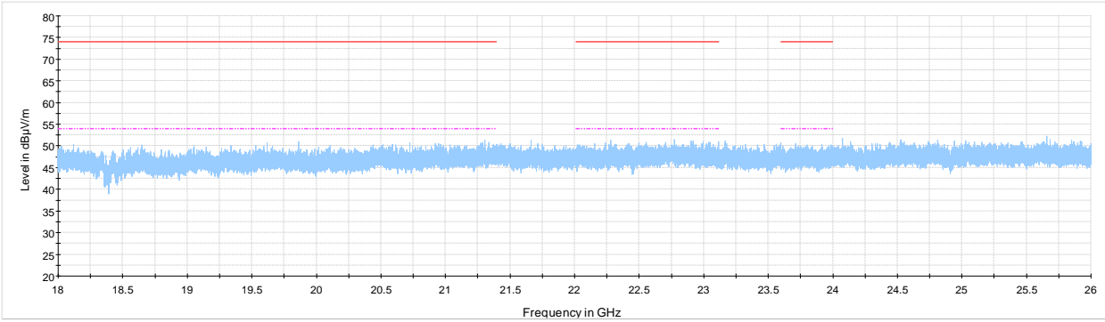
Figure 7.6-10: Radiated spurious emissions 18-26 GHz mid channel
