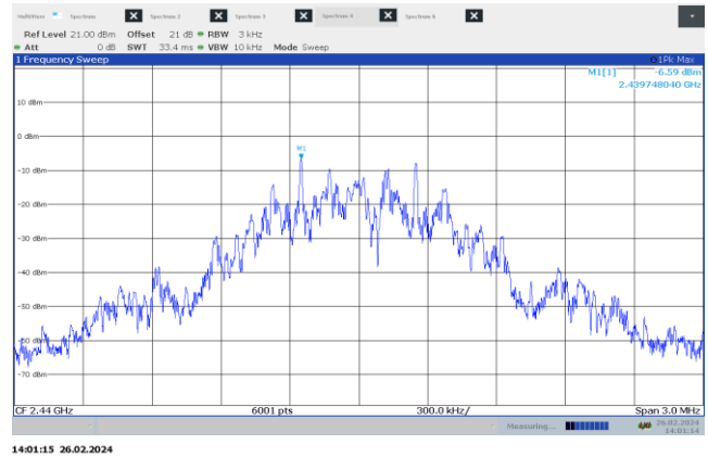
Figure 7.7-2: PSD on mid channel – 1 MHz
