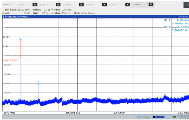
Figure 7.6-23: Conducted spurious emissions on low channel – 2 MHz
