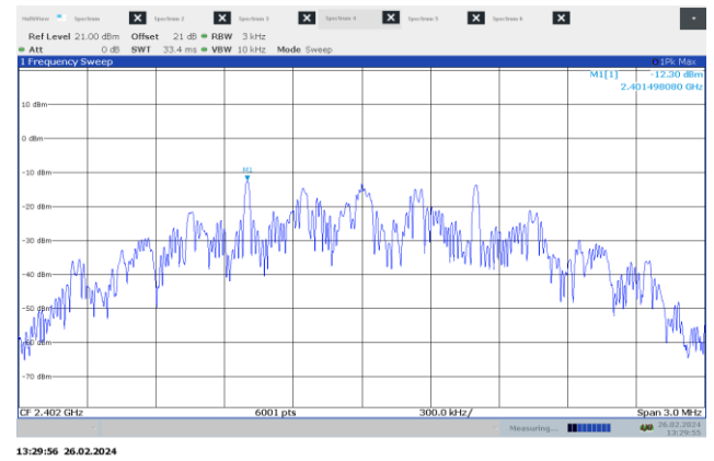
Figure 7.7-4: PSD on low channel – 2 MHz
