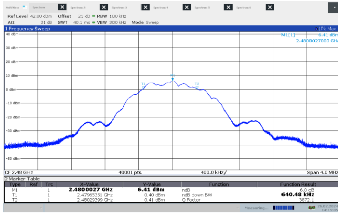
Figure 7.4-3: 6 dB bandwidth on high channel – 1 MHz BW
