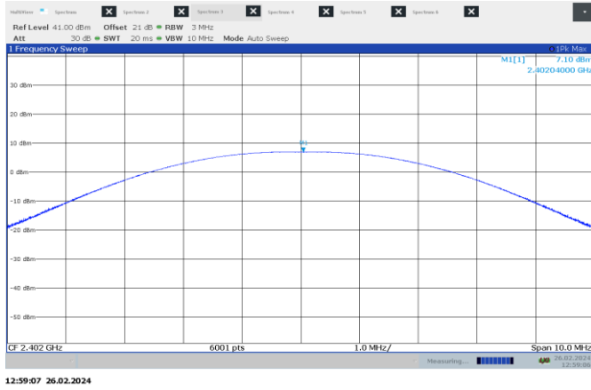
Figure 7.5-1: Output power on low channel – 1 MHz BW
