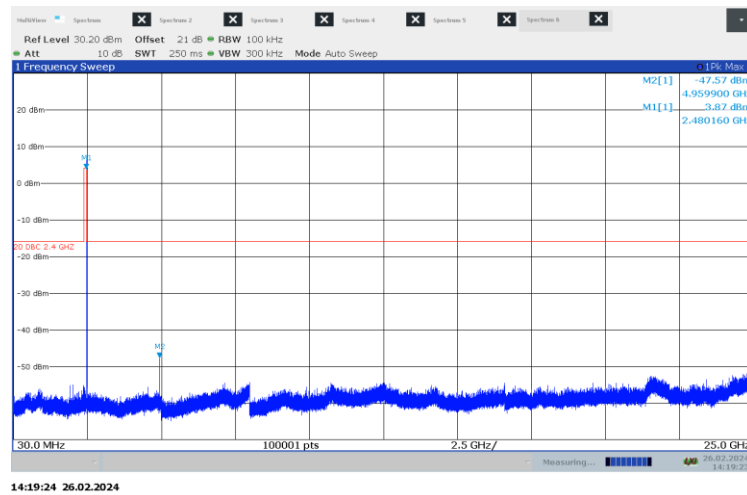
Figure 7.6-22: Conducted spurious emissions on high channel – 1 MHz
