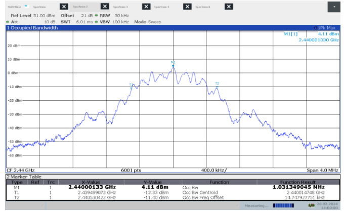
Figure 7.4-8: 99% occupied bandwidth on mid channel – 1 MHz BW
