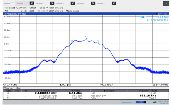
Figure 7.4-2: 6 dB bandwidth on mid channel – 1 MHz BW
