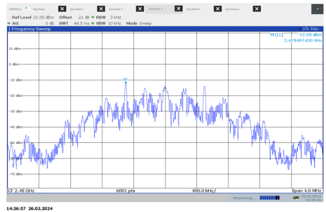
Figure 7.7-4: PSD on high channel – 2 MHz
