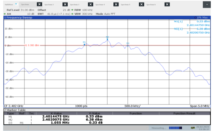
Figure 7.4-4: 6 dB bandwidth on low channel – 2 MHz BW
