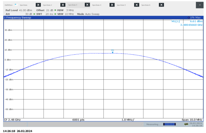
Figure 7.5-6: Output power on high channel – 2 MHz BW
