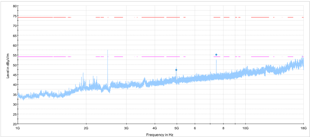
PRJ52103466 RE 1-18 GHz, BLE, high ch., PRK002001 rev A — Preview Result 1-PK+ — FCC 15.209 and RSS-Gen Restricted bands peak limits — FCC 15.209 and RSS-Gen Restricted bands average limits ◆ Final_Result PK+
