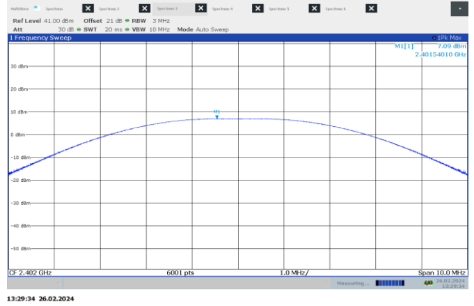
Figure 7.5-4: Output power on low channel – 2 MHz BW
