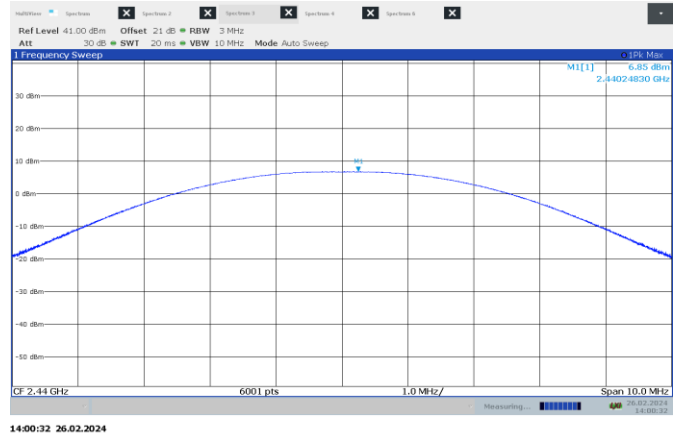
Figure 7.5-2: Output power on mid channel – 1 MHz BW
