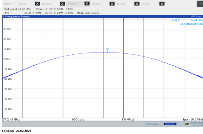
Figure 7.5-3: Output power on high channel – 1 MHz BW
