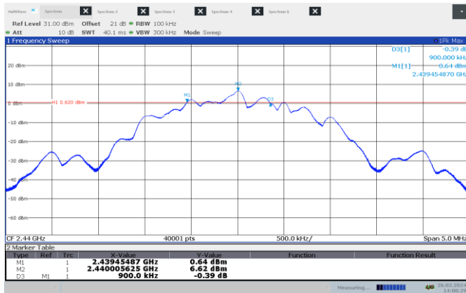
Figure 7.4-5: 6 dB bandwidth on mid channel – 2 MHz BW
