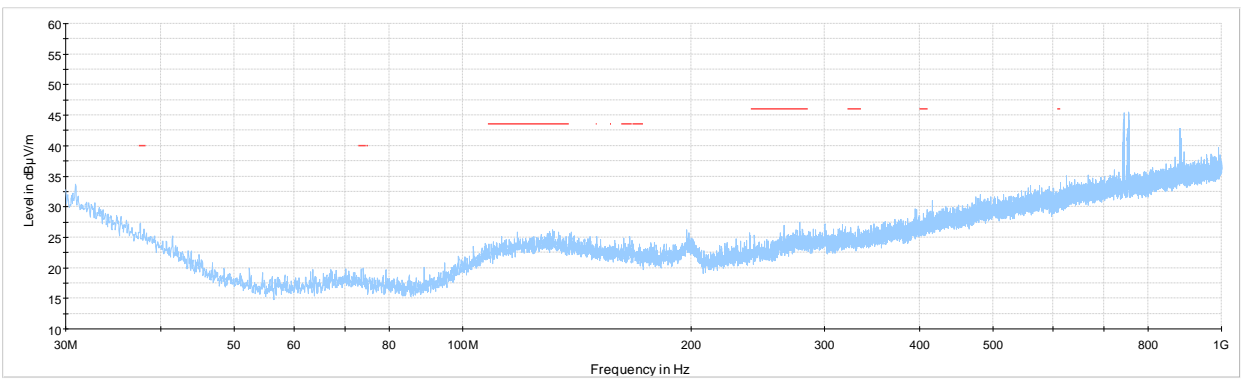
Figure 7.6-4: Radiated spurious emissions 30-1000 MHz mid channel
