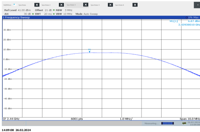
Figure 7.5-5: Output power on mid channel – 2 MHz BW
