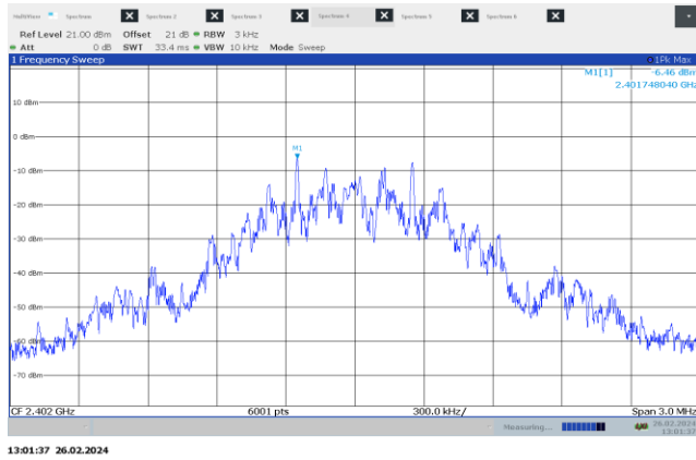
Figure 7.7-1: PSD on low channel – 1 MHz
