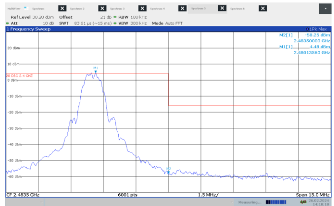
Figure 7.6-15: Conducted non-restricted band edge emissions at 2483.5 MHz – 1 MHz
