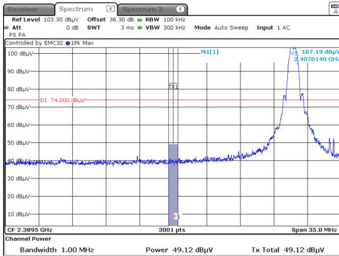
Figure 7.6-12: Radiated band edge spurious emissions at 2390 MHz Peak – 1 MHz
