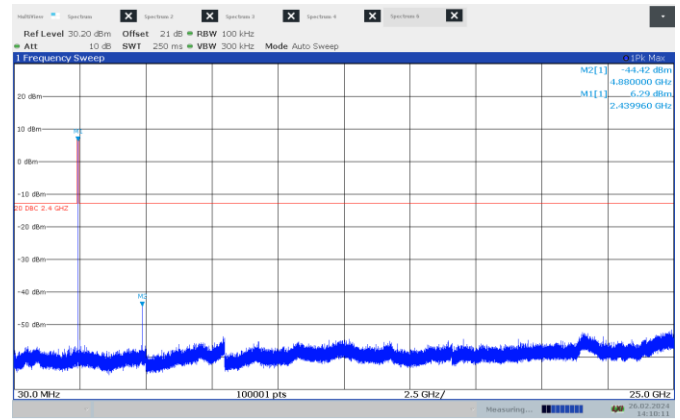
Figure 7.6-24: Conducted spurious emissions on mid channel – 2 MHz
