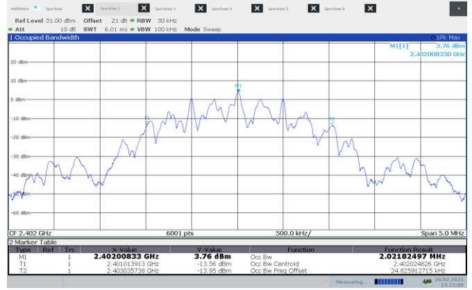
Figure 7.4-10: 99% occupied bandwidth on low channel – 2 MHz BW
