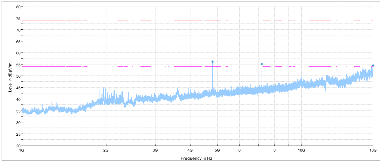
PRJ52103466 RE 1-18 GHz, BLE, low ch., PRK002001 rev A Preview Result 1-PK+ FCC 15.209 and RSS-Gen Restricted bands peak limits FCC 15.209 and RSS-Gen Restricted bands average limits Final_Result PK+
