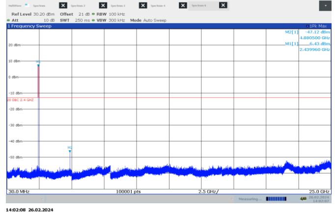
Figure 7.6-21: Conducted spurious emissions on mid channel – 1 MHz
