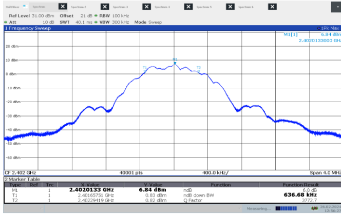
Figure 7.4-1: 6 dB bandwidth on low channel – 1 MHz BW
