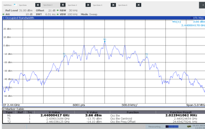
Figure 7.4-11 99% occupied bandwidth on mid channel – 2 MHz BW
