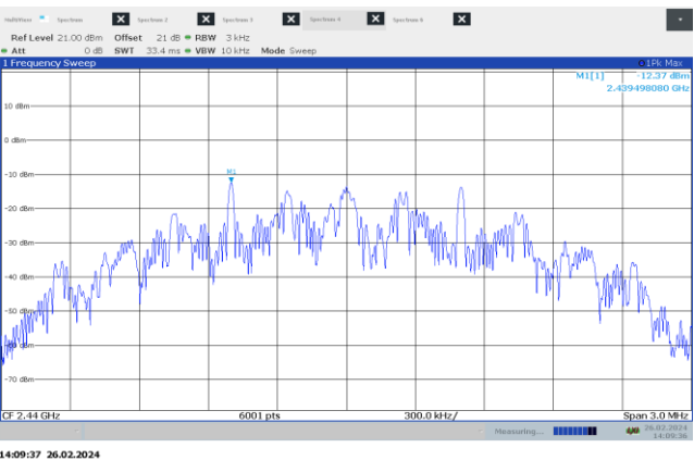
Figure 7.7-4: PSD on mid channel – 2 MHz
