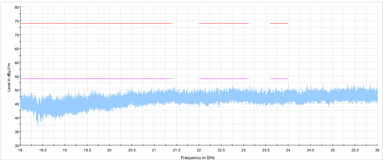
PRJ52103466 RE 18-26 GHz, BLE, low ch., PRK002001 rev A — Preview Result 1-PK+ — FCC 15.209 and RSS-Gen Restricted bands peak limits — FCC 15.209 and RSS-Gen Restricted bands average limits
