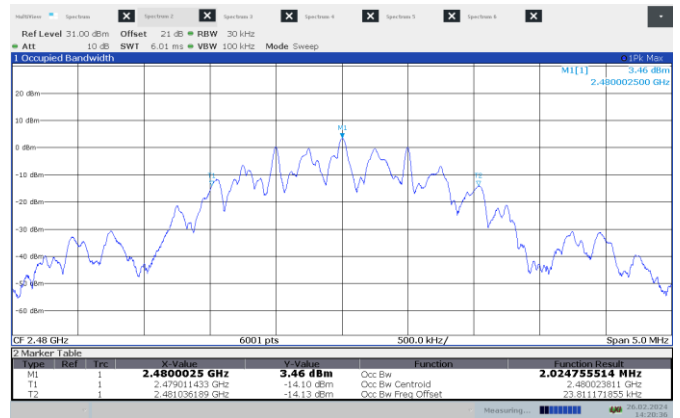
Figure 7.4-12: 99% occupied bandwidth on high channel – 2 MHz BW
