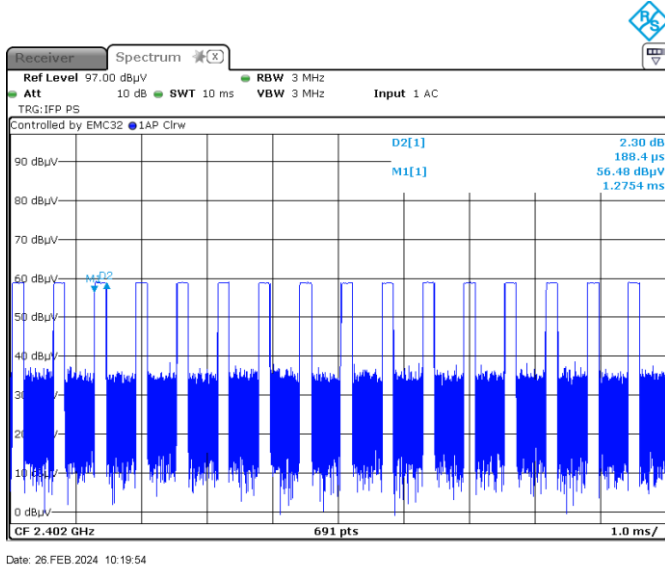
Figure 7.6-1: Pulse width
