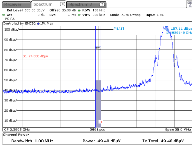
Figure 7.6-16: Radiated band edge spurious emissions at 2390 MHz Peak – 2 MHz
