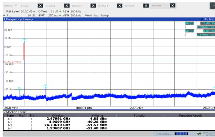
Figure 7.6-25: Conducted spurious emissions on high channel – 2 MHz
