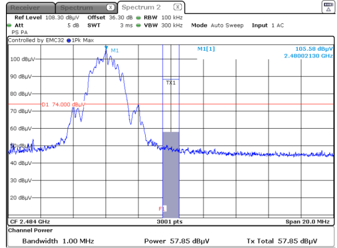
Figure 7.6-17: Radiated band edge spurious emissions at 2483.5 MHz Peak – 2 MHz
