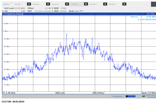
Figure 7.7-3: PSD on high channel – 1 MHz
