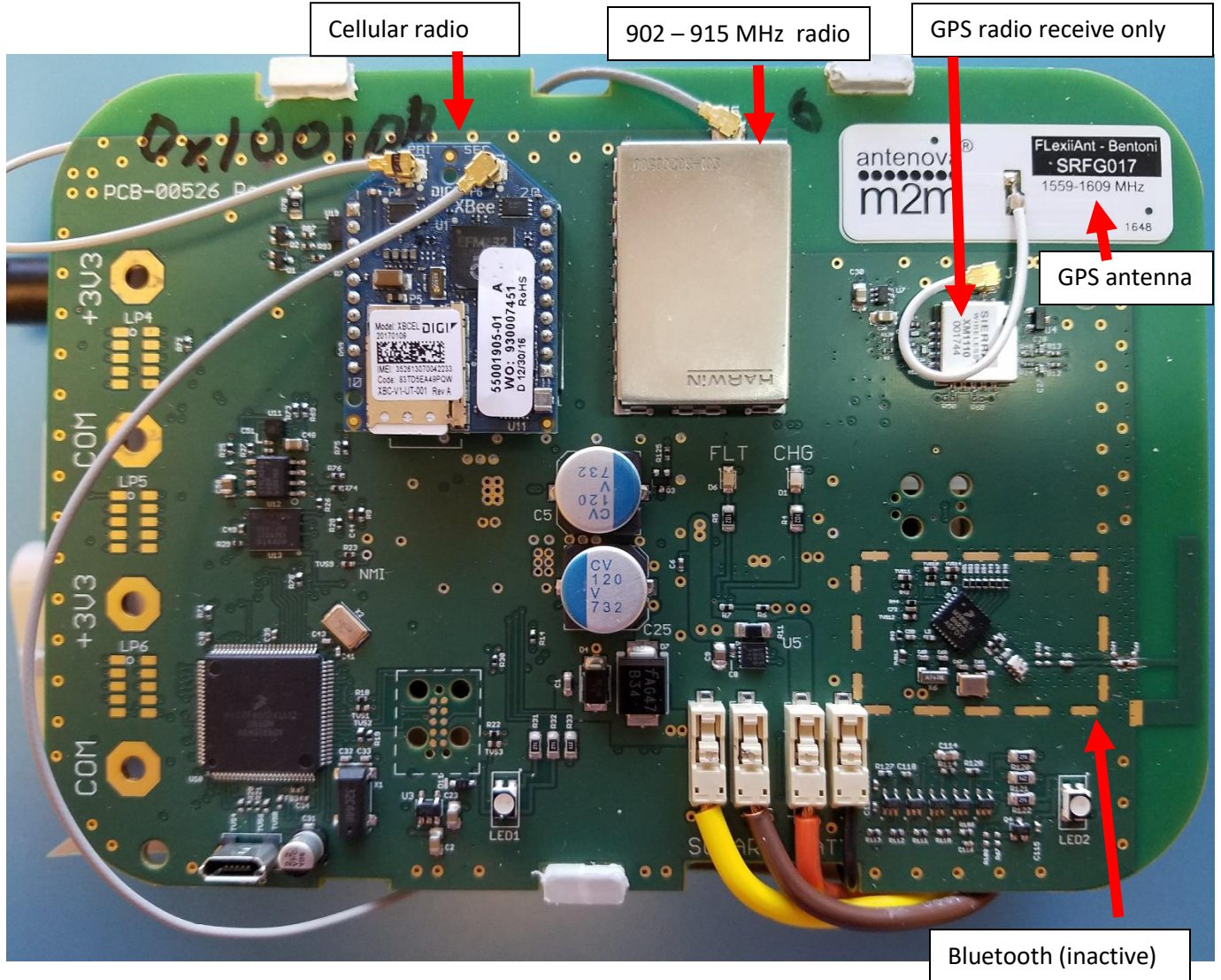
Figure 2 – Circuit board assembly with shield
