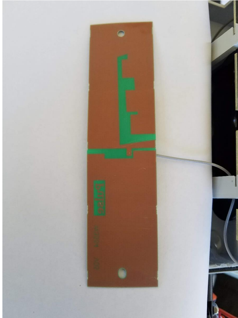
Figure 7 - Cellular antenna, opposite side
