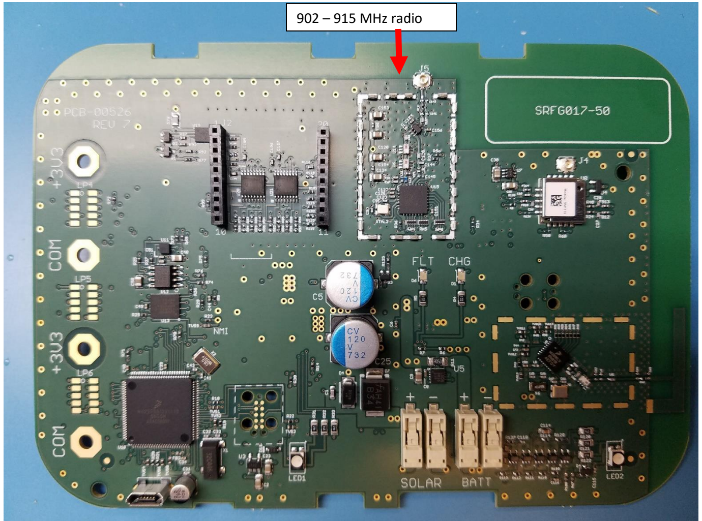
Figure 1- Circuit board assembly without shield
