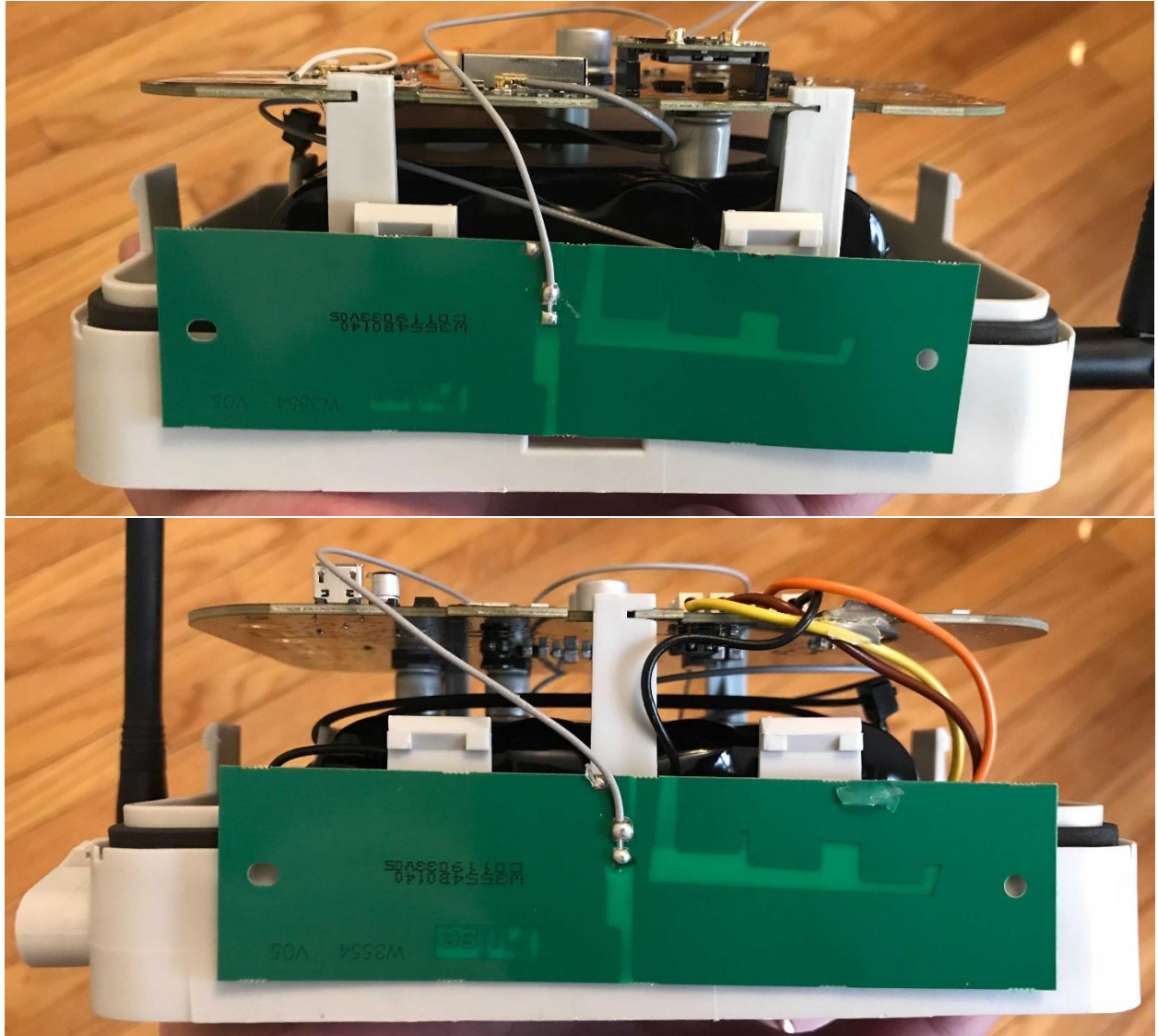
Figure 6 - Cellular antenna, both sides, 2 of the same antenna
