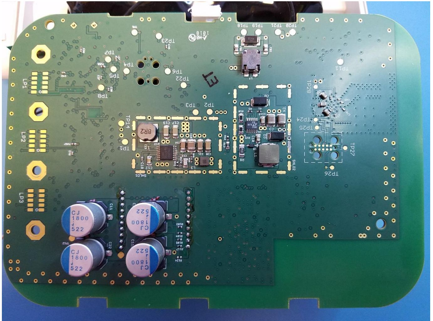
Figure 3 - Circuit board bottom
