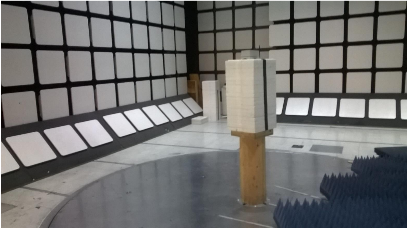
Figure 5 - Test Setup for 1- 10 GHz
