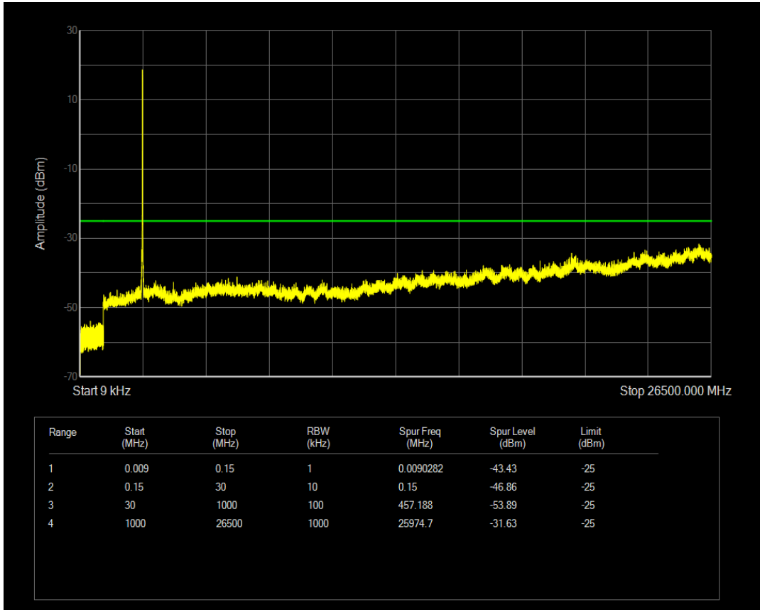
Band41 QAM16 BW=15MHz Channel=41115 RB Size=1 Position=#0
