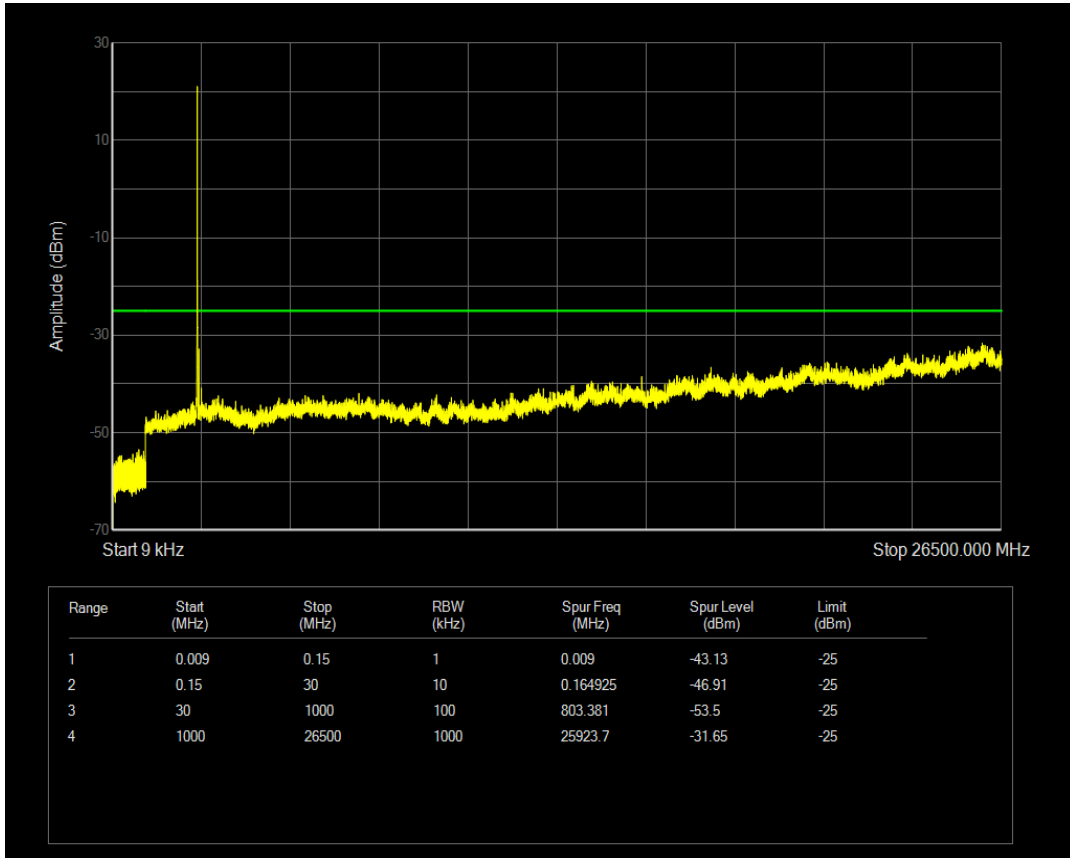
Band41 QAM16 BW=5MHz Channel=40115 RB Size=25 Position=#0
