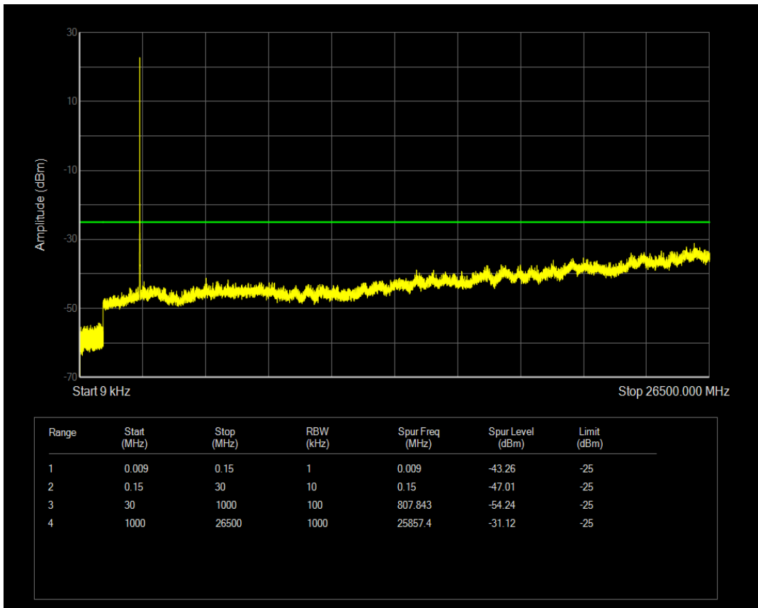
Band41 QAM16 BW=5MHz Channel=40115 RB Size=1 Position=#0
