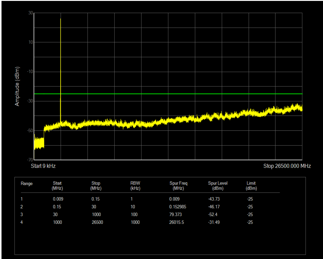
Band41 QAM16 BW=10MHz Channel=41140 RB Size=1 Position=#0
