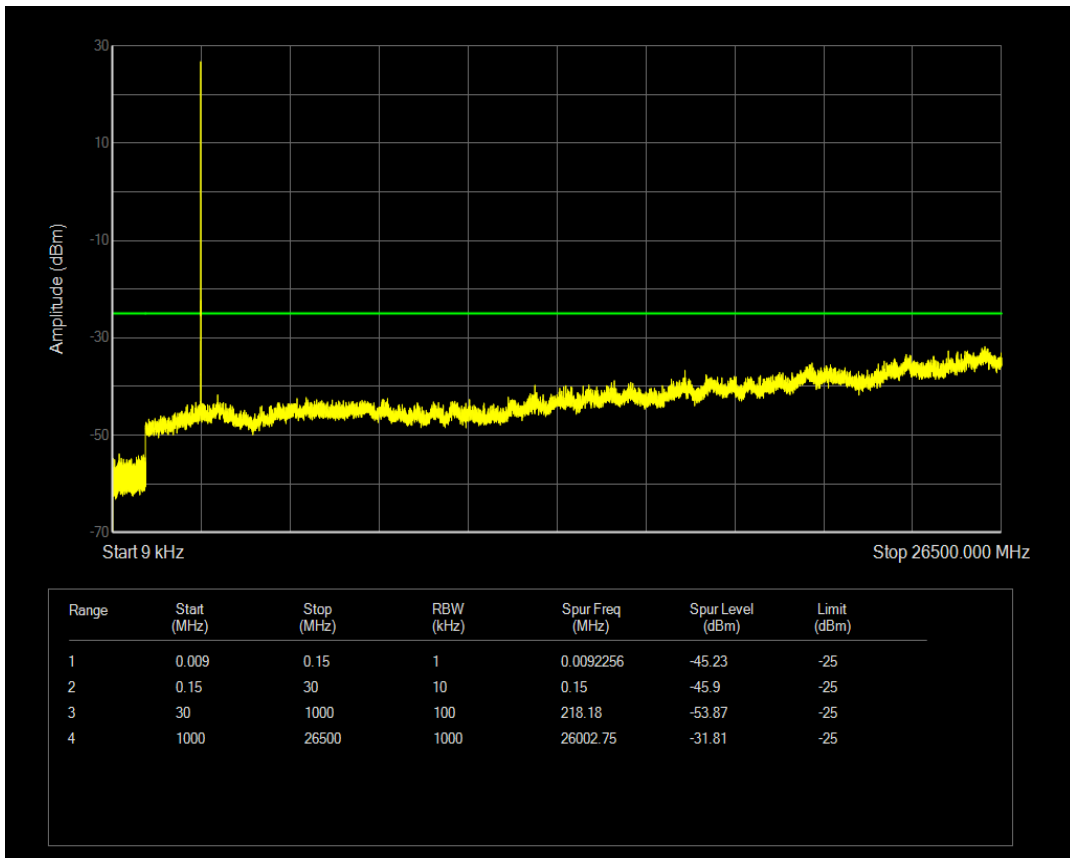
Band41 QAM16 BW=5MHz Channel=41165 RB Size=25 Position=#0
