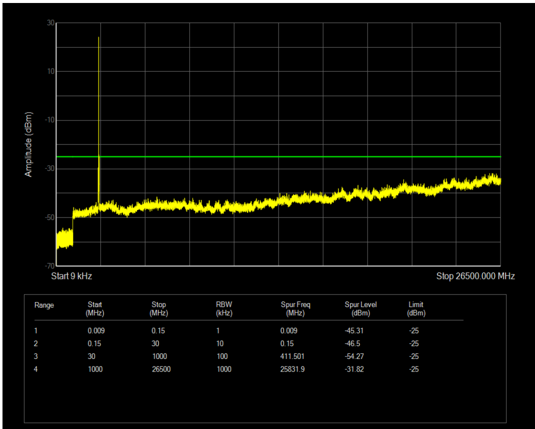
Band41 QAM16 BW=20MHz Channel=40190 RB Size=100 Position=#0
