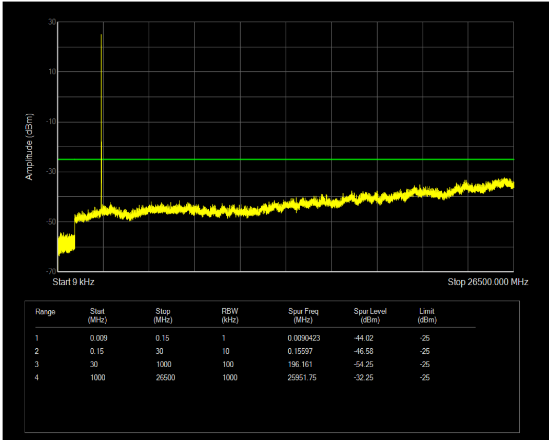
Band41 QAM16 BW=10MHz Channel=40140 RB Size=1 Position=#0
