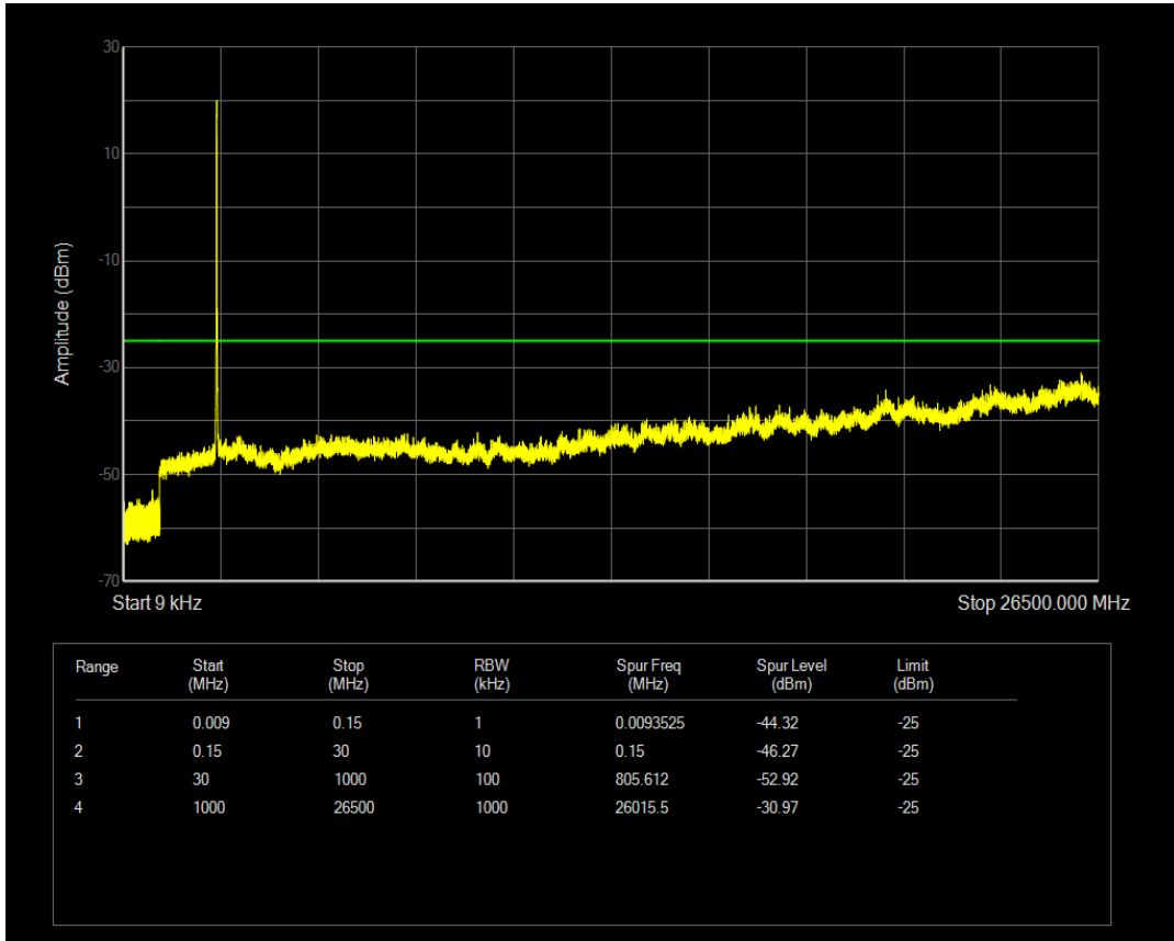
Band41 QAM16 BW=15MHz Channel=40165 RB Size=1 Position=#0
