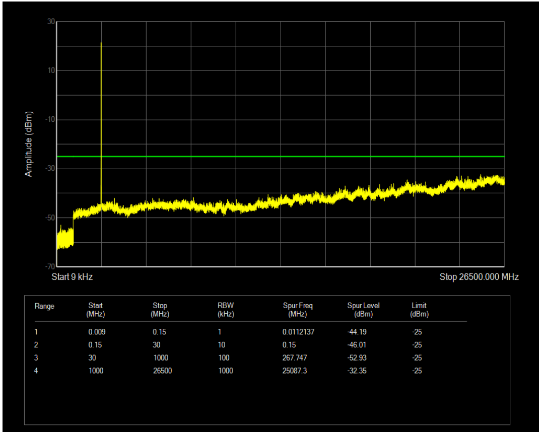
Band41 QAM16 BW=5MHz Channel=41165 RB Size=1 Position=#0
