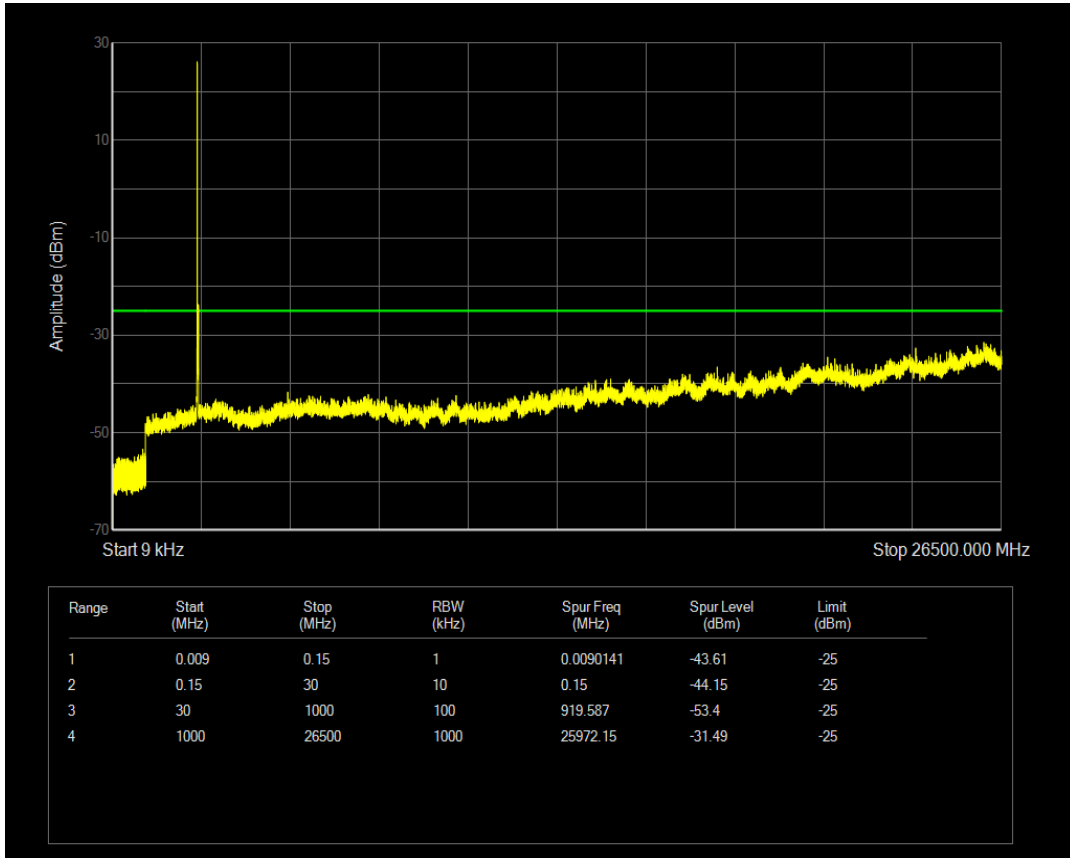
Band41 QAM16 BW=20MHz Channel=40190 RB Size=1 Position=#0
