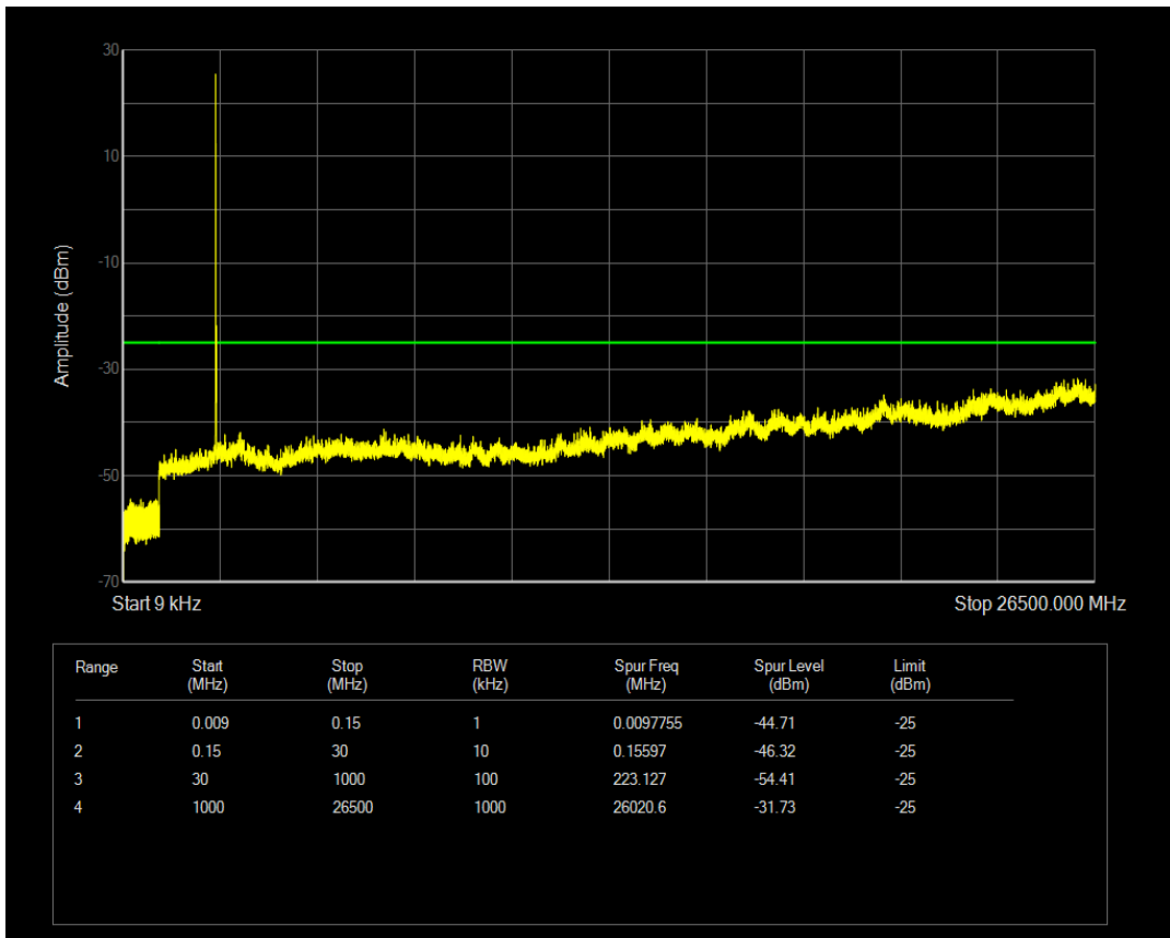
Band41 QAM16 BW=10MHz Channel=40140 RB Size=50 Position=#0
