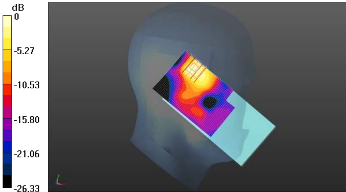
0 dB = 0.350 W/kg = -4.56 dBW/kg
