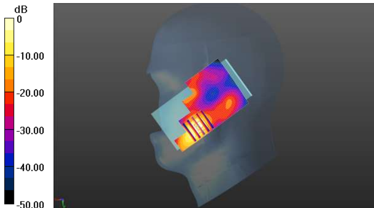
0 dB = 0.0496 W/kg = -13.05 dBW/kg
